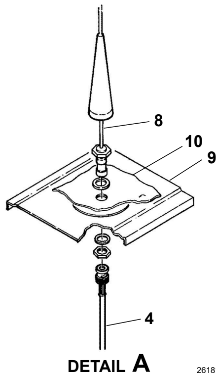
EMERGENCY LOCATOR TRANSMITTER INSTALLATION - FRENCH CERTIFIED AIRPLANES Figure 04. (Sheet 1)
