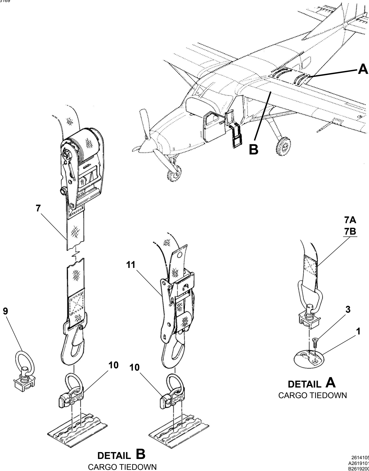
CARGO TIEDOWN INSTALLATION Figure 01. (Sheet 1)
