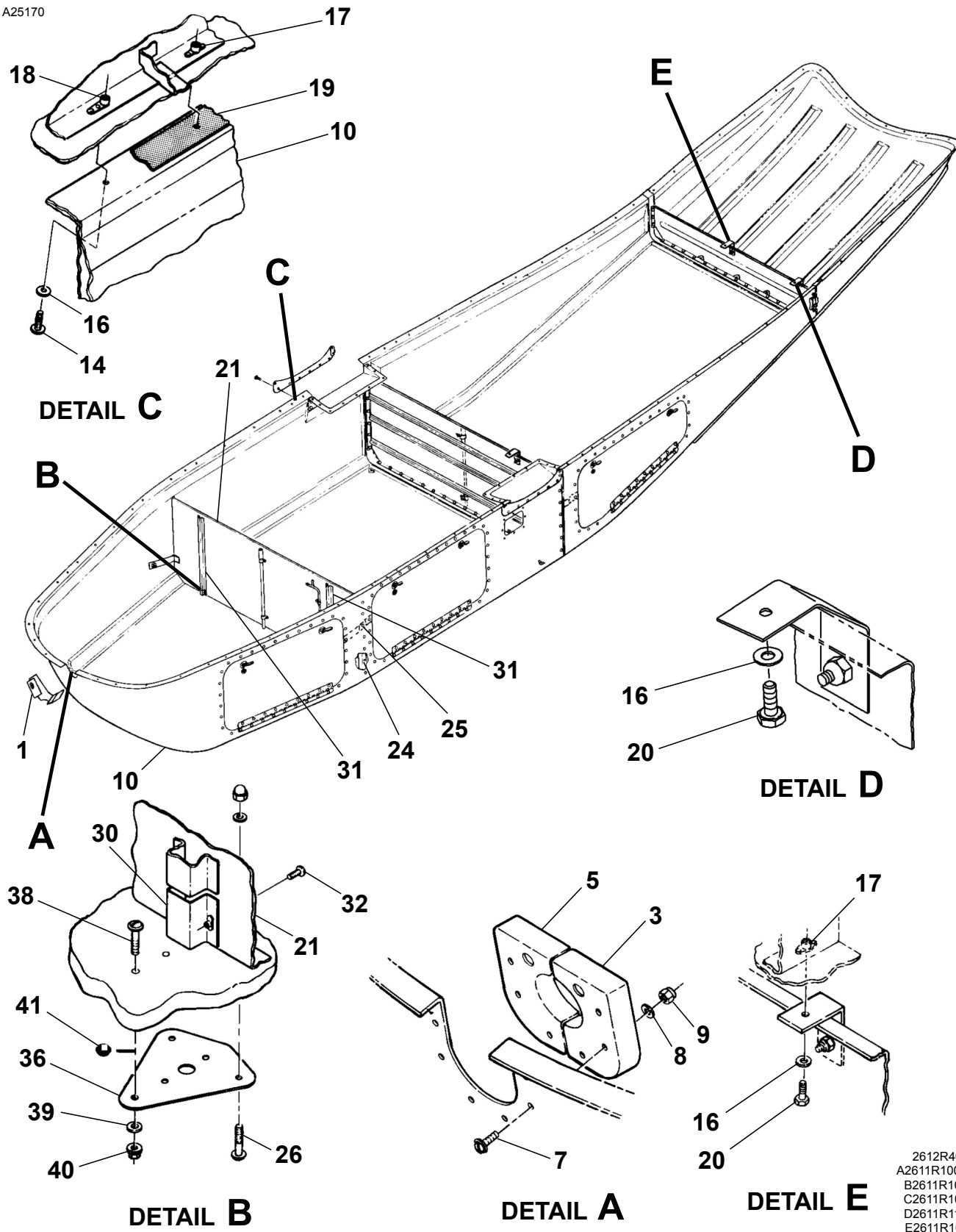
CARGO POD INSTALLATION Figure 01. (Sheet 1)
