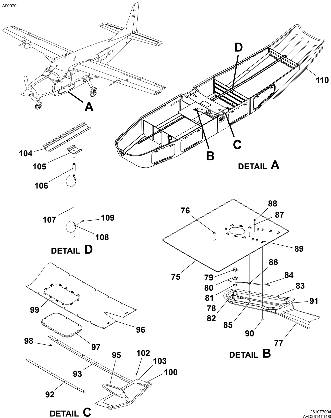
CARGO POD FIELD INSTALLATION Figure 02A. (Sheet 2)
