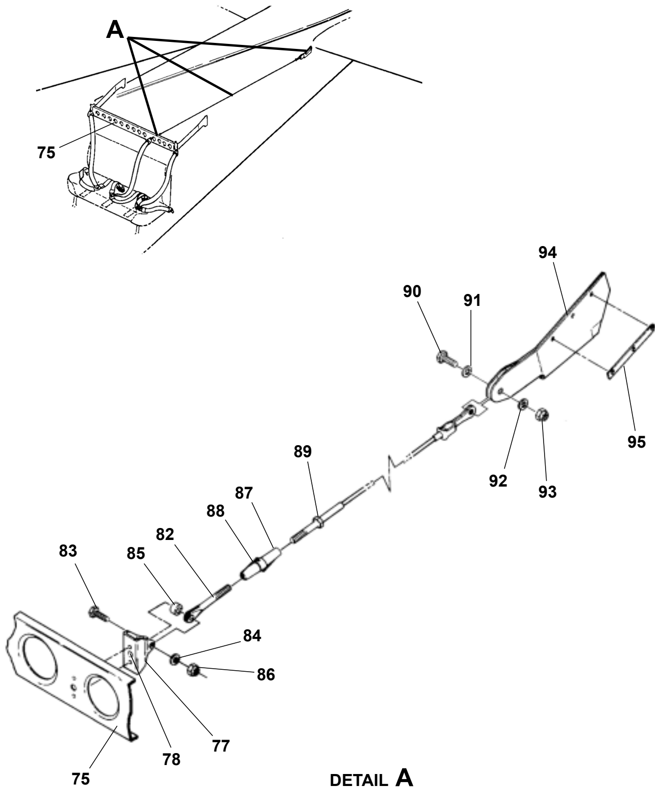
SEAT AND SHOULDER HARNESS INSTALLATION - 3 PASSENGER Figure 01. (Sheet 2)
