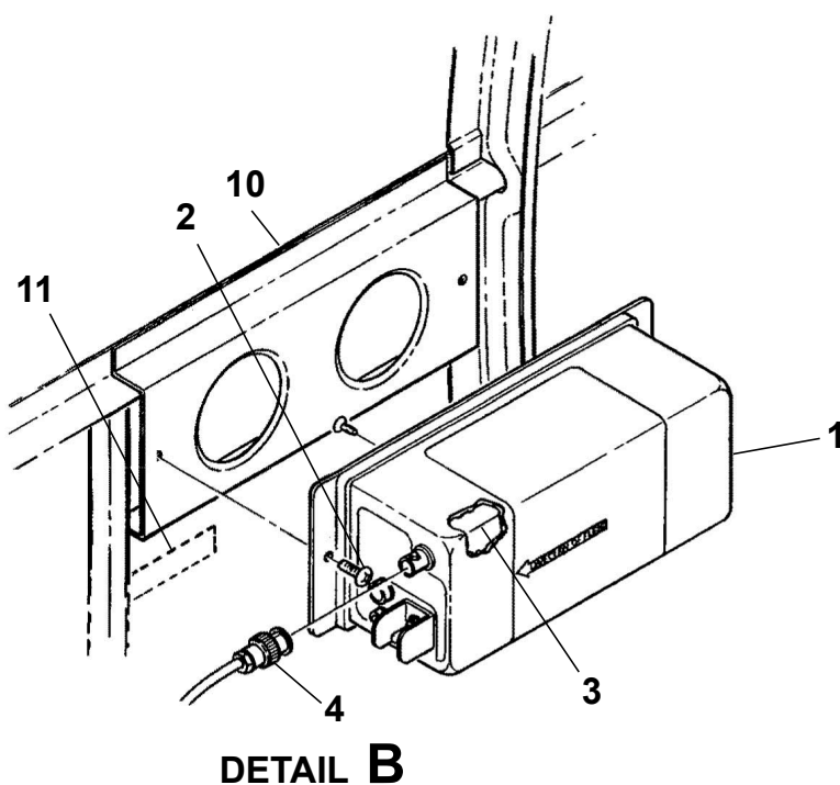
EMERGENCY LOCATOR TRANSMITTER INSTALLATION - FRENCH CERTIFIED AIRPLANES Figure 04. (Sheet 1)
