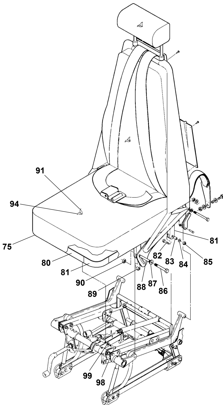
SEAT ASSEMBLY - PILOT AND COPILOT Figure 01. (Sheet 2)
