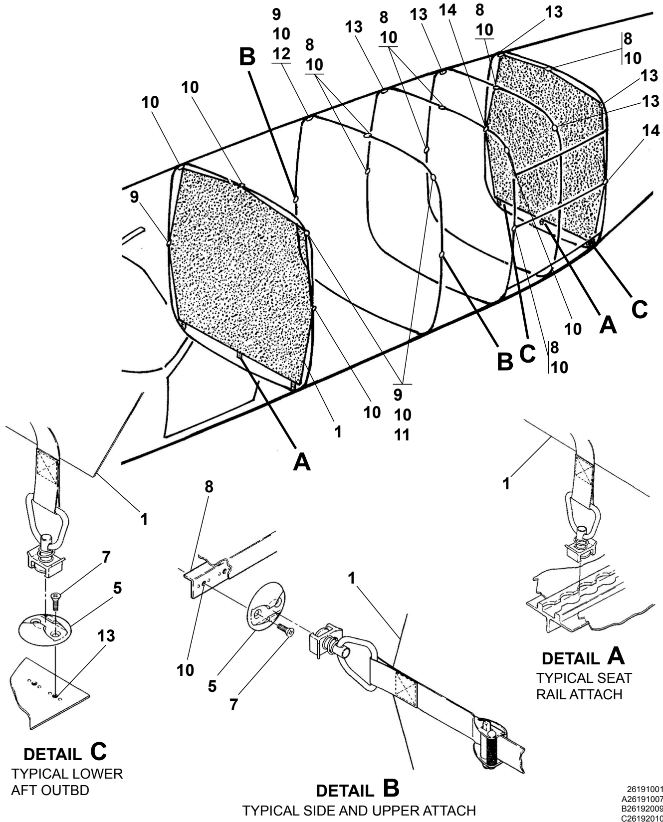
CARGO PARTITION INSTALLATION - NOT APPLICABLE TO PASSENGER VERSION Figure 01. (Sheet 1)
