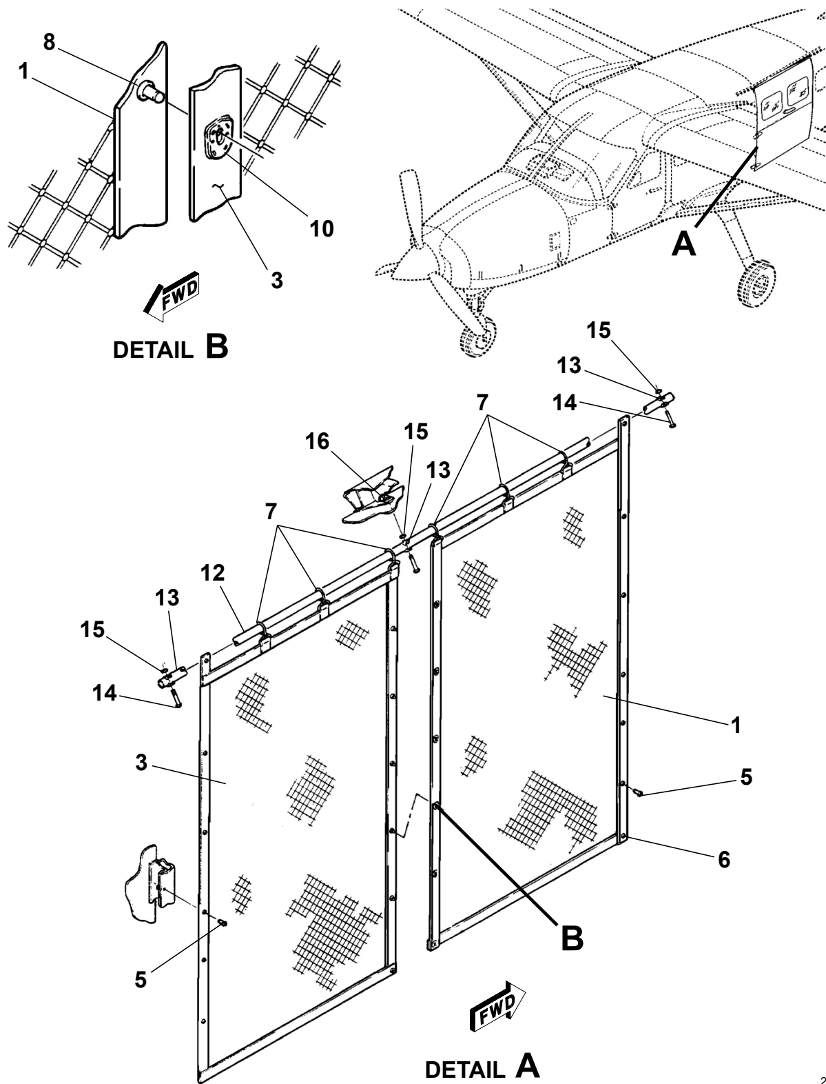
RESTRAINING NET INSTALLATION - CARGO DOOR Figure 01. (Sheet 1)
