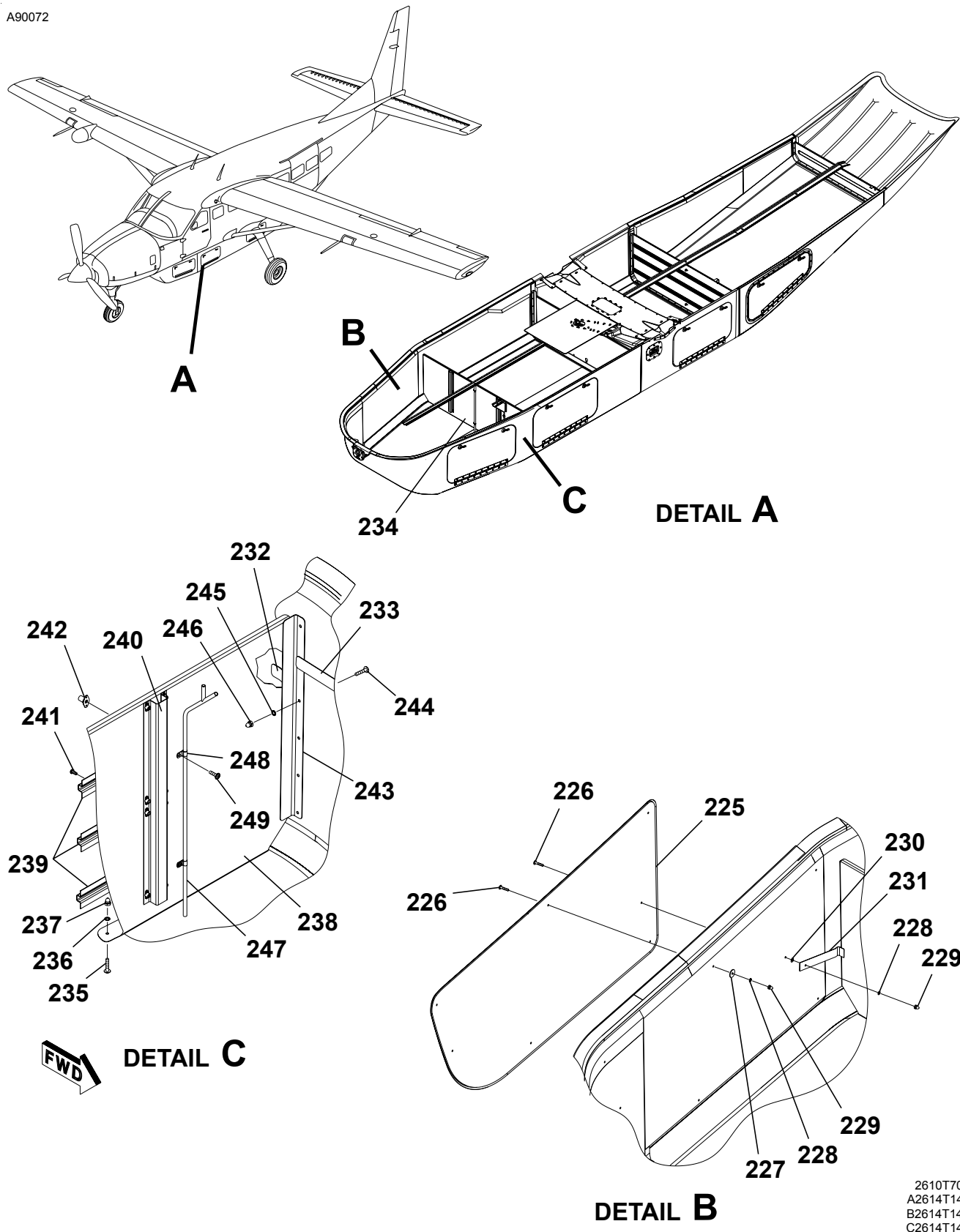
CARGO POD FIELD INSTALLATION Figure 02A. (Sheet 4)
