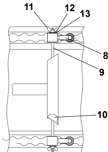
VIEW B-B
