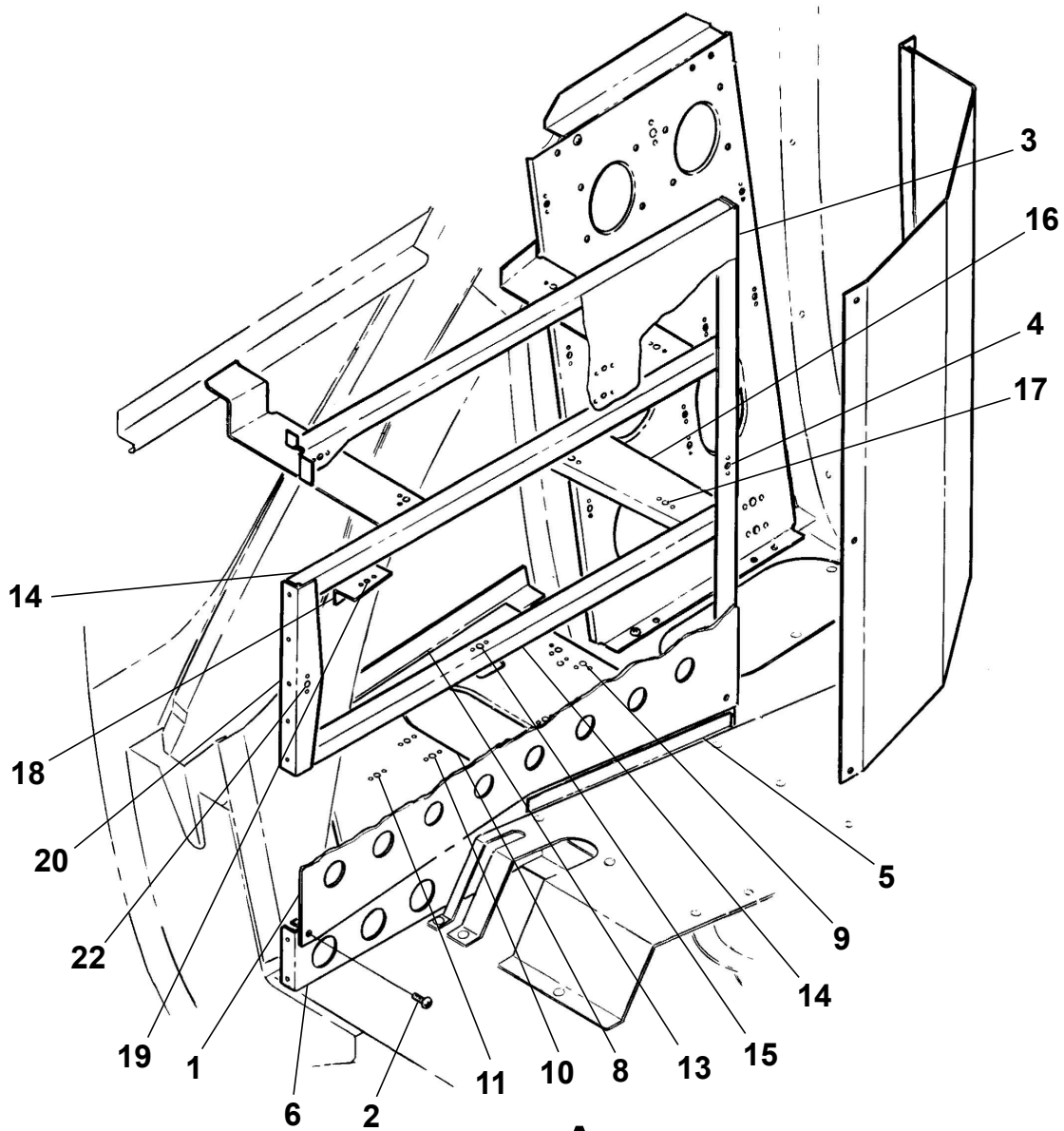
AVIONICS RACK INSTALLATION Figure 01. (Sheet 1)
