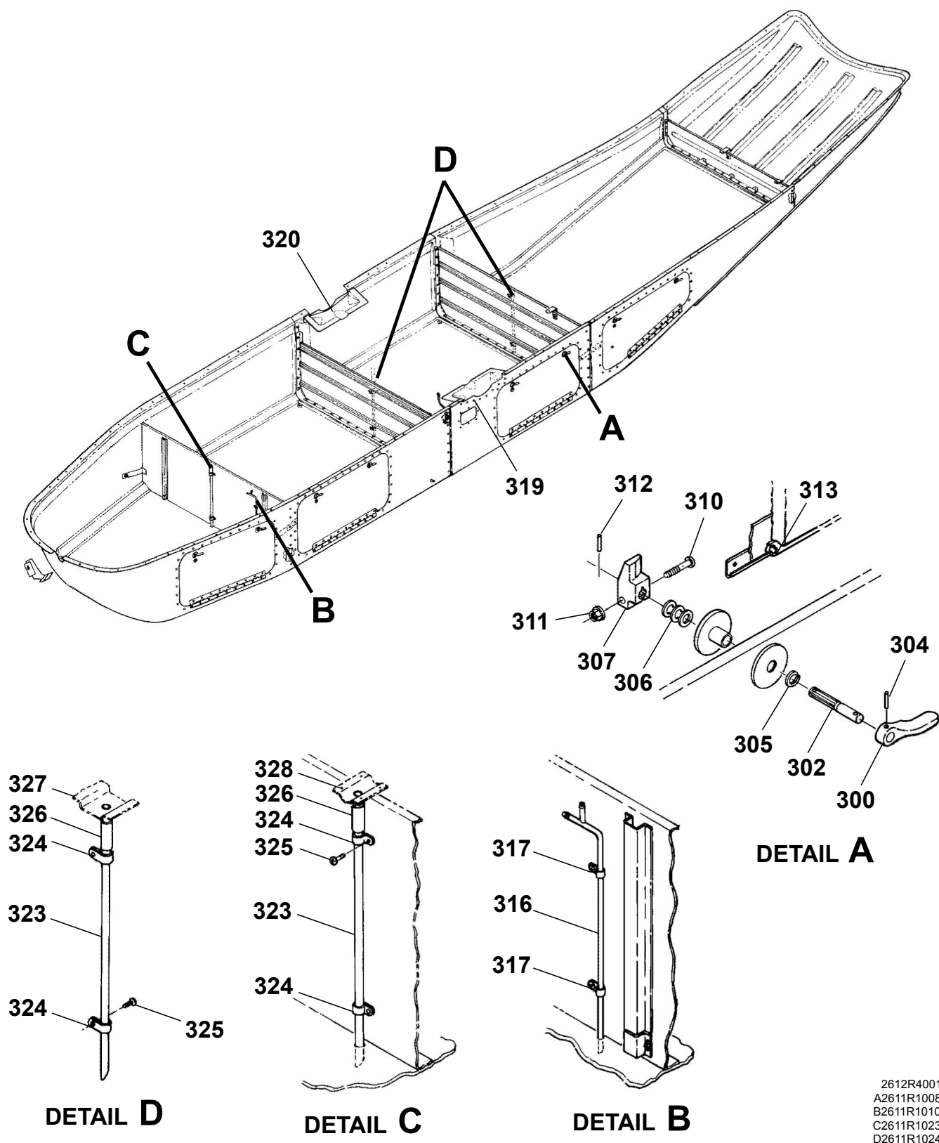
CARGO POD INSTALLATION Figure 02. (Sheet 5)
