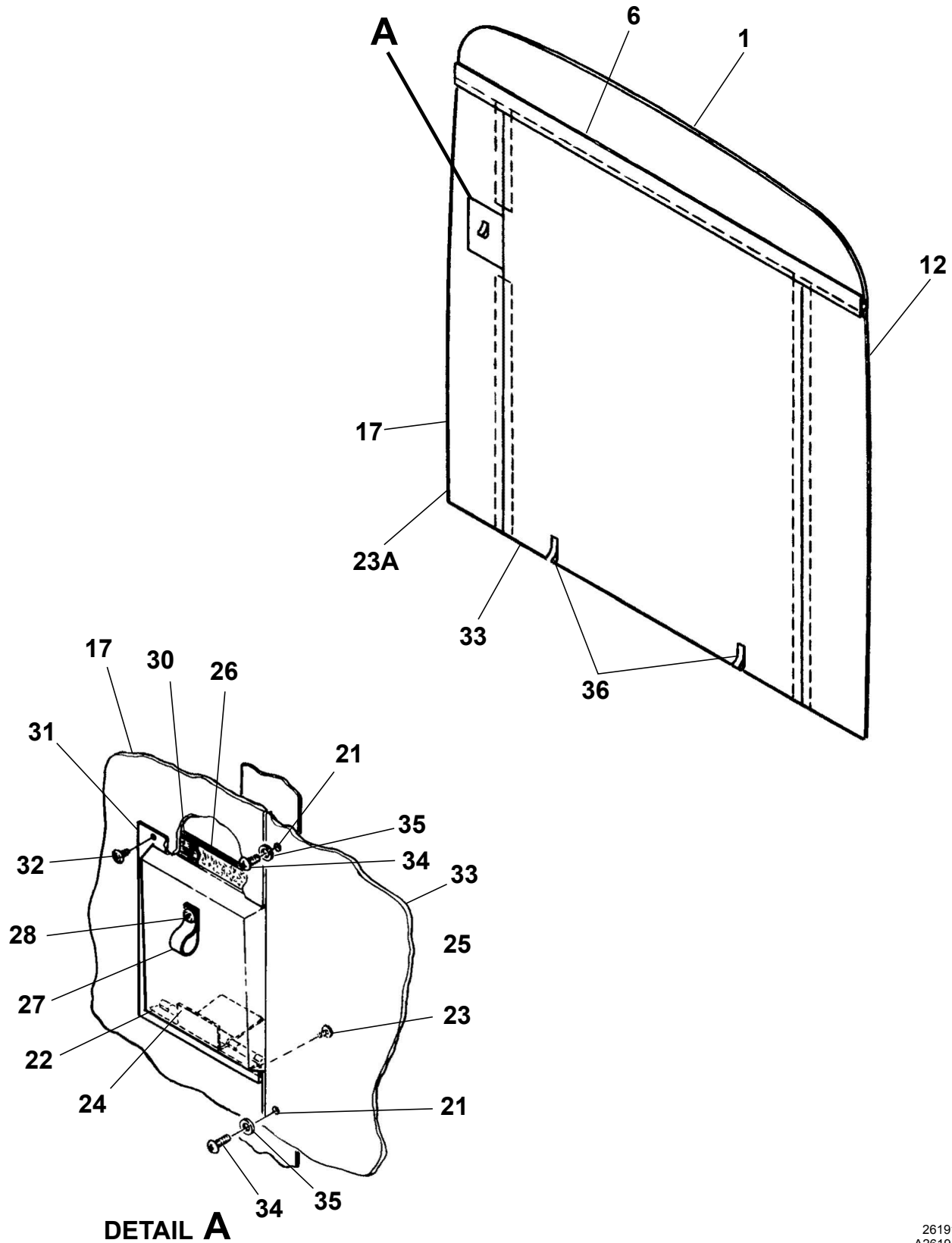
REAR CARGO COMPARTMENT WALL UPHOLSTERY Figure 01. (Sheet 1)
