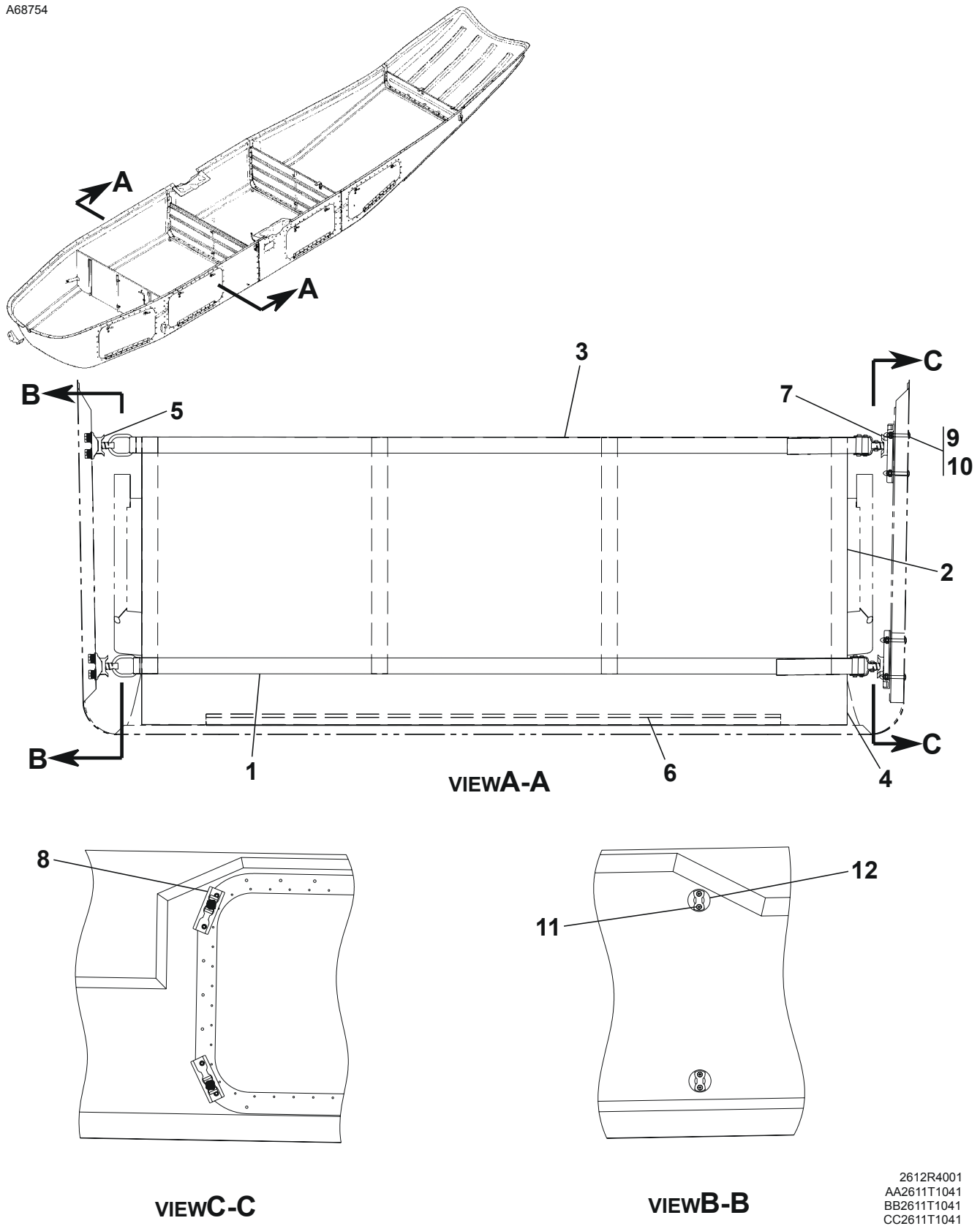
TKS CARGO NET INSTALLATION Figure 03. (Sheet 1)
