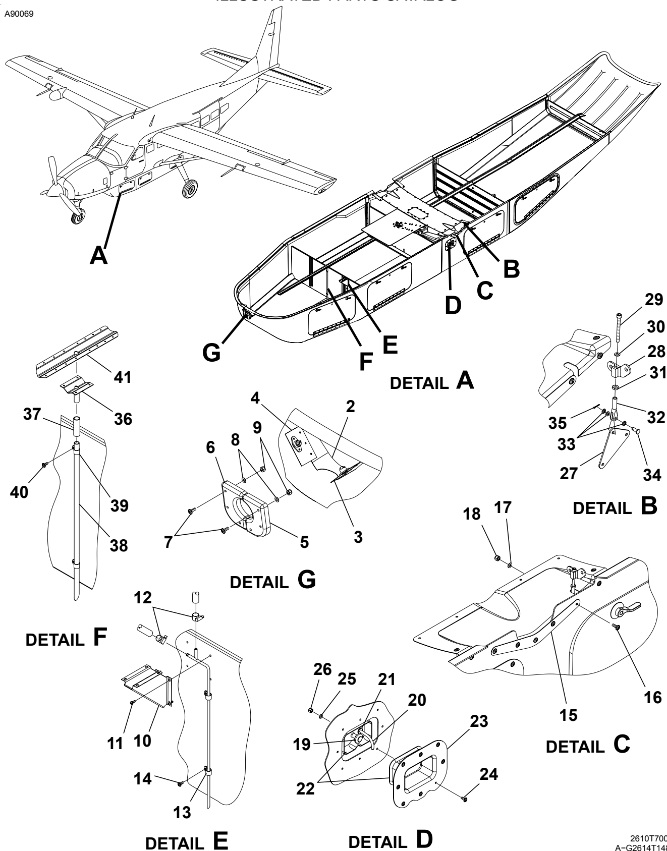
CARGO POD FIELD INSTALLATION Figure 02A. (Sheet 1)
