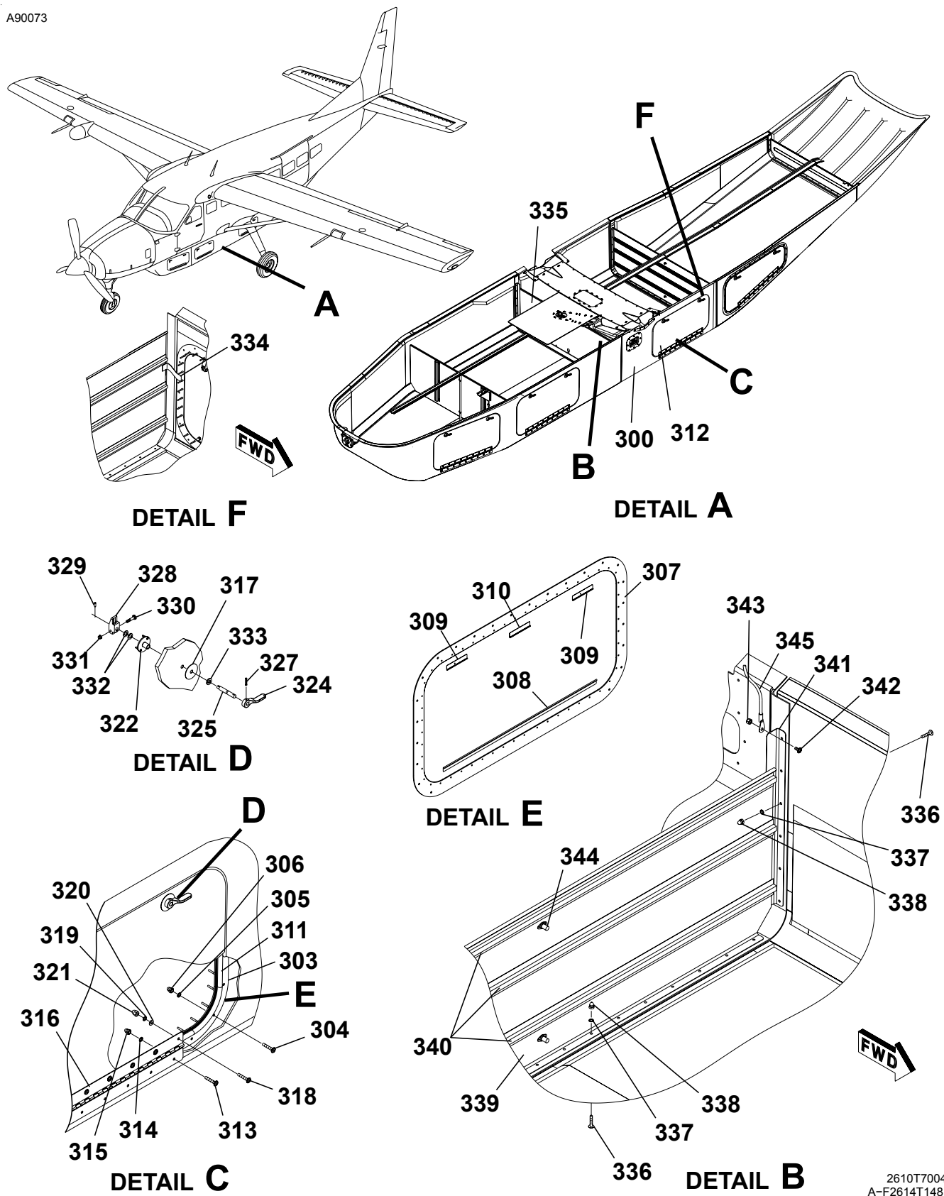
CARGO POD FIELD INSTALLATION Figure 02A. (Sheet 5)
