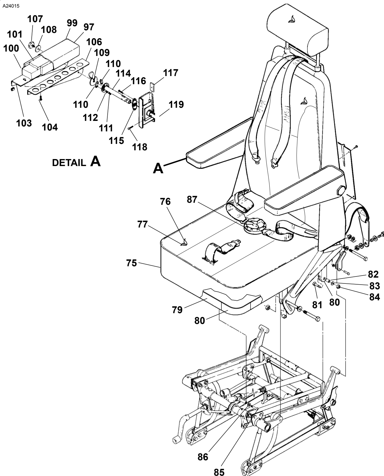
SEAT ASSEMBLY - PILOT AND COPILOT WITH ARMREST Figure 02A. (Sheet 2)
