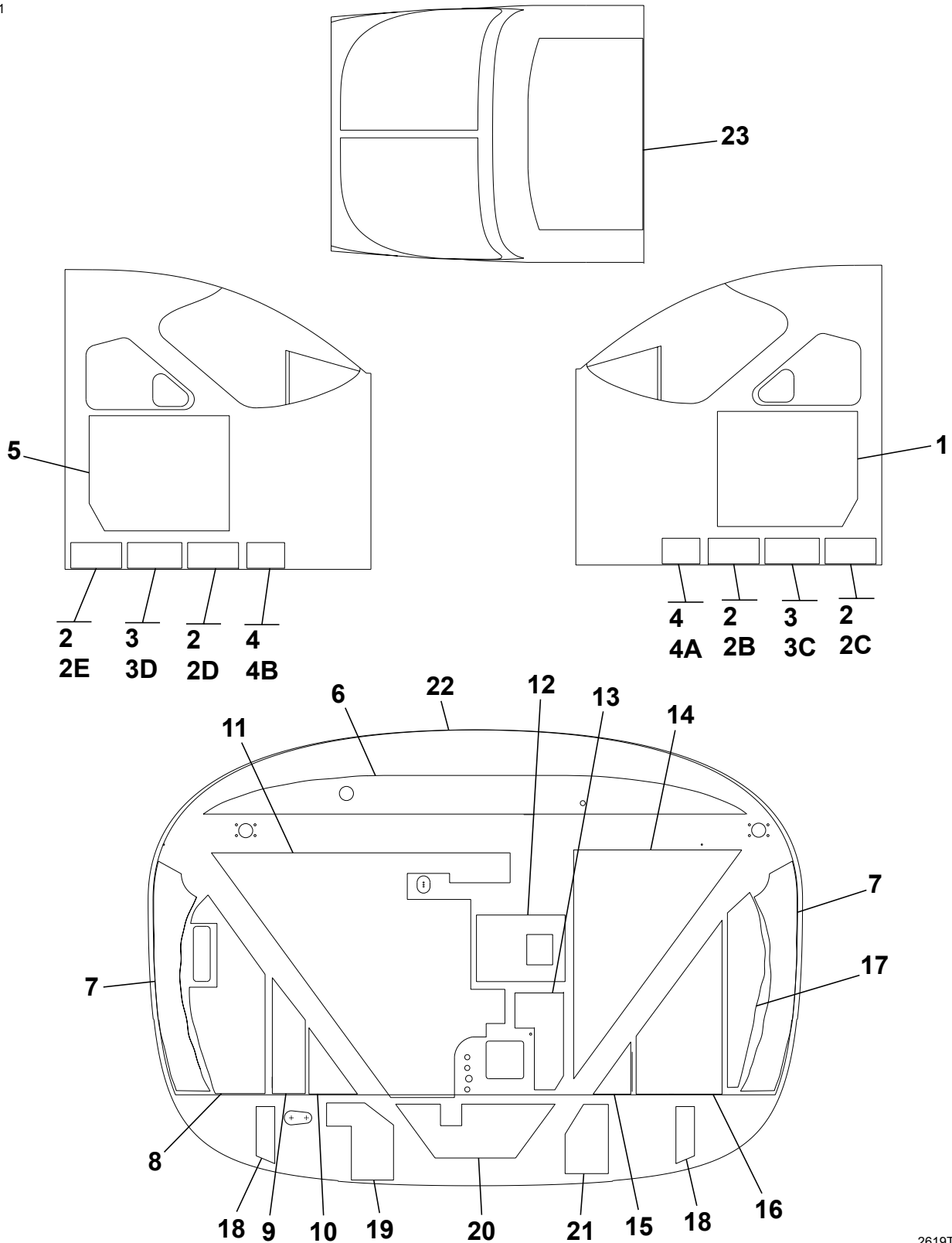
FIREWALL VIEW LOOKING FORWARD INSULATION - CARGO VERSION Figure 05. (Sheet 1)
