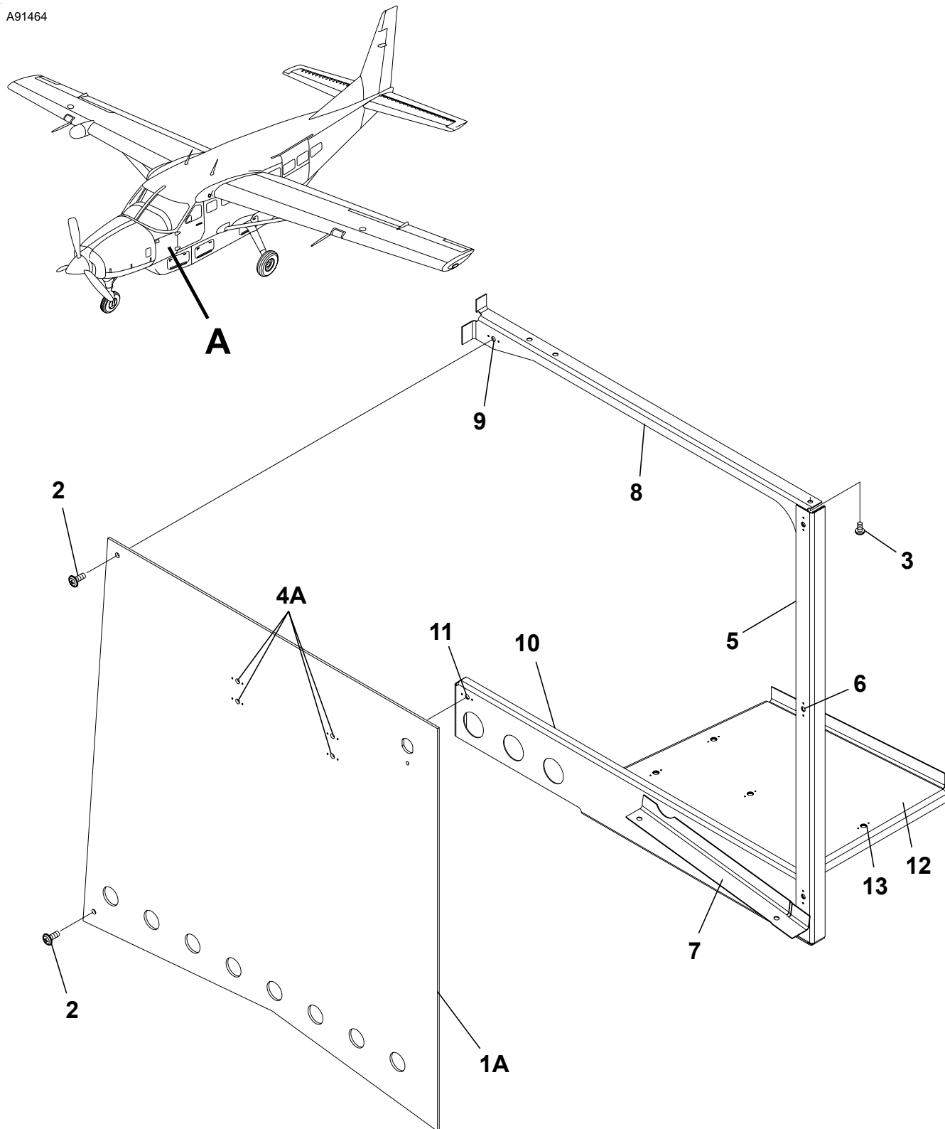
DETAIL A AVIONICS RACK INSTALLATION Figure 02. (Sheet 1)
