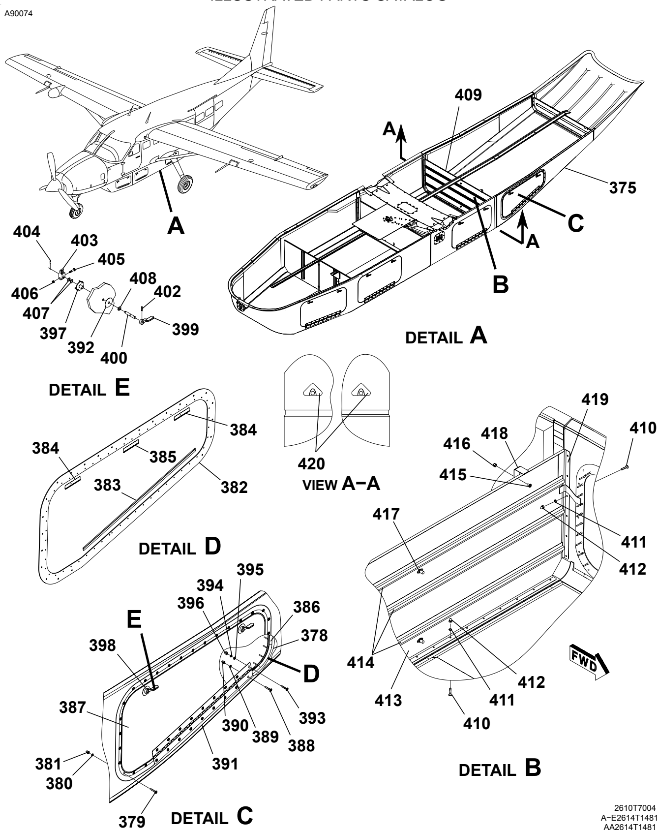
CARGO POD FIELD INSTALLATION Figure 02A. (Sheet 6)
