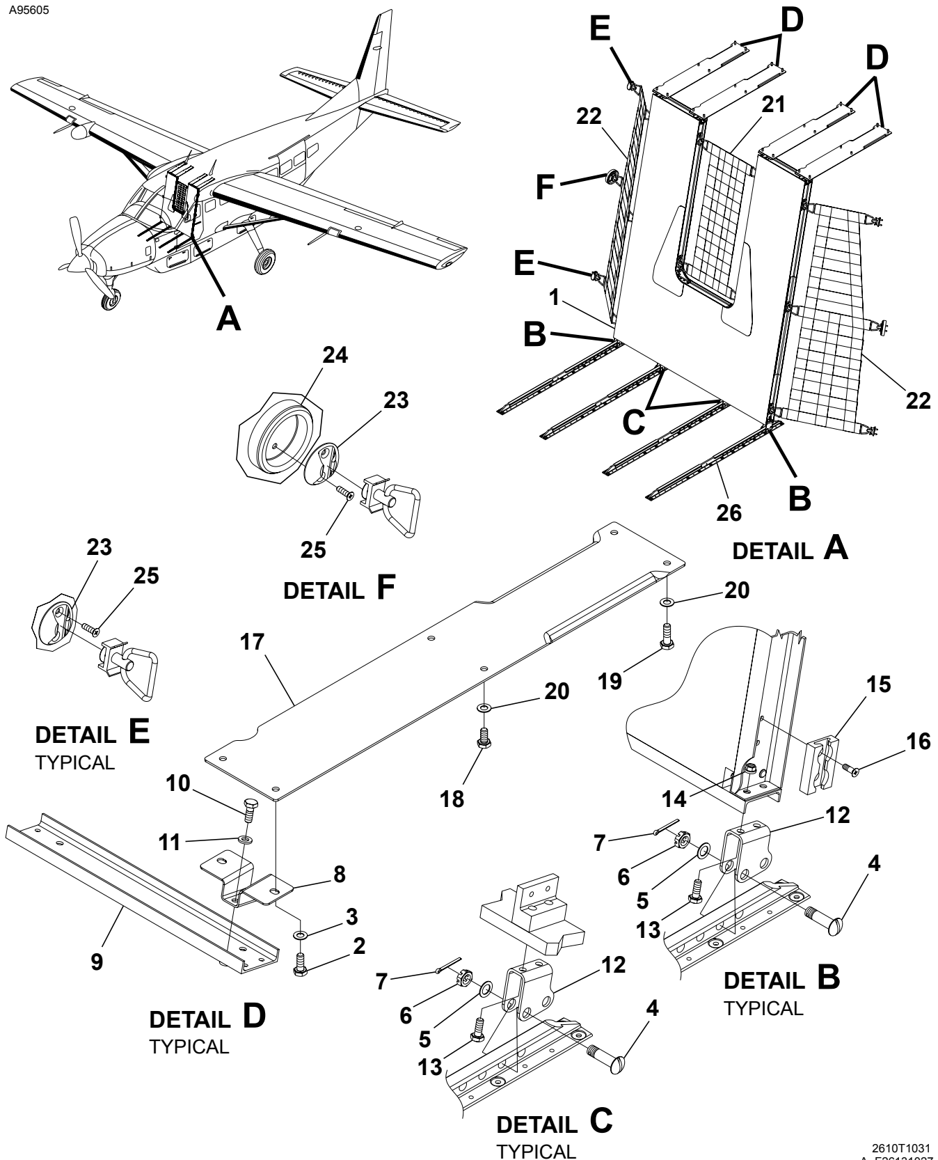
CARGO BARRIER INSTALLATION Figure 03. (Sheet 1)
