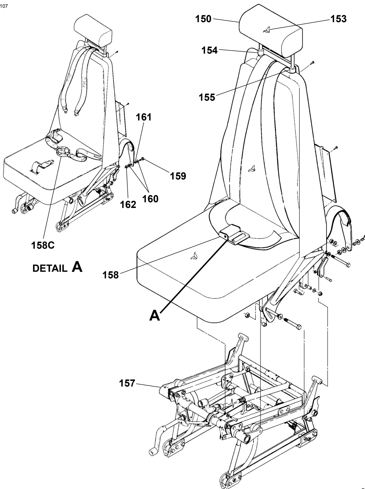
SEAT ASSEMBLY - PILOT AND COPILOT Figure 01. (Sheet 3)
