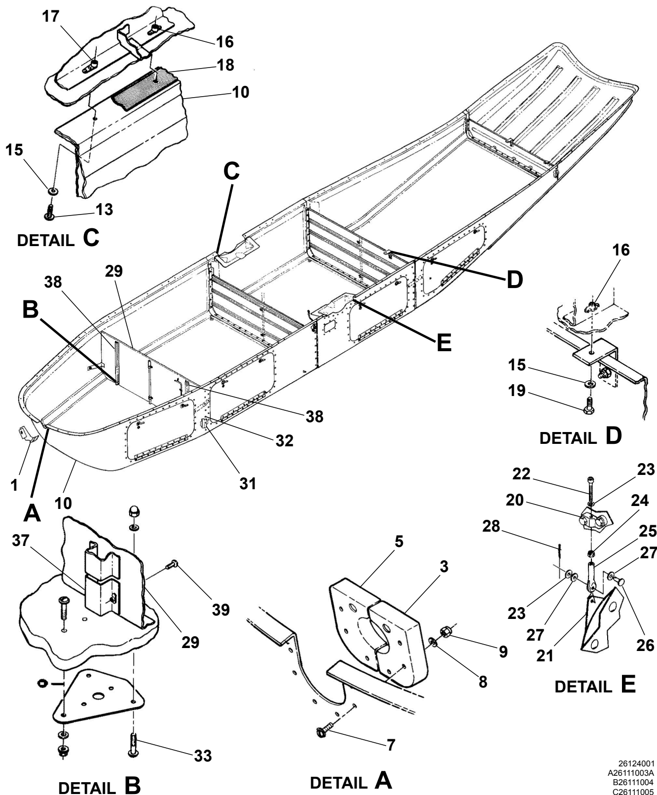
CARGO POD INSTALLATION Figure 02. (Sheet 1)
