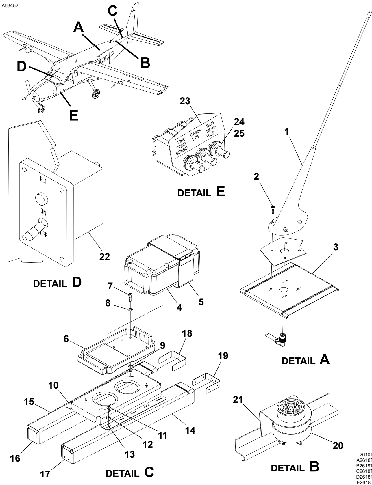
EMERGENCY LOCATOR TRANSMITTER - ME-406 Figure 07. (Sheet 1)
