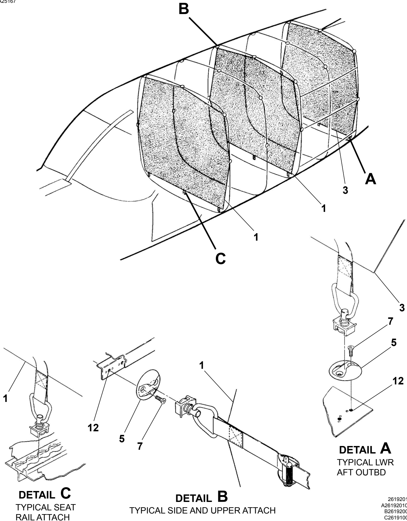
CARGO PARTITION INSTALLATION Figure 02. (Sheet 1)
