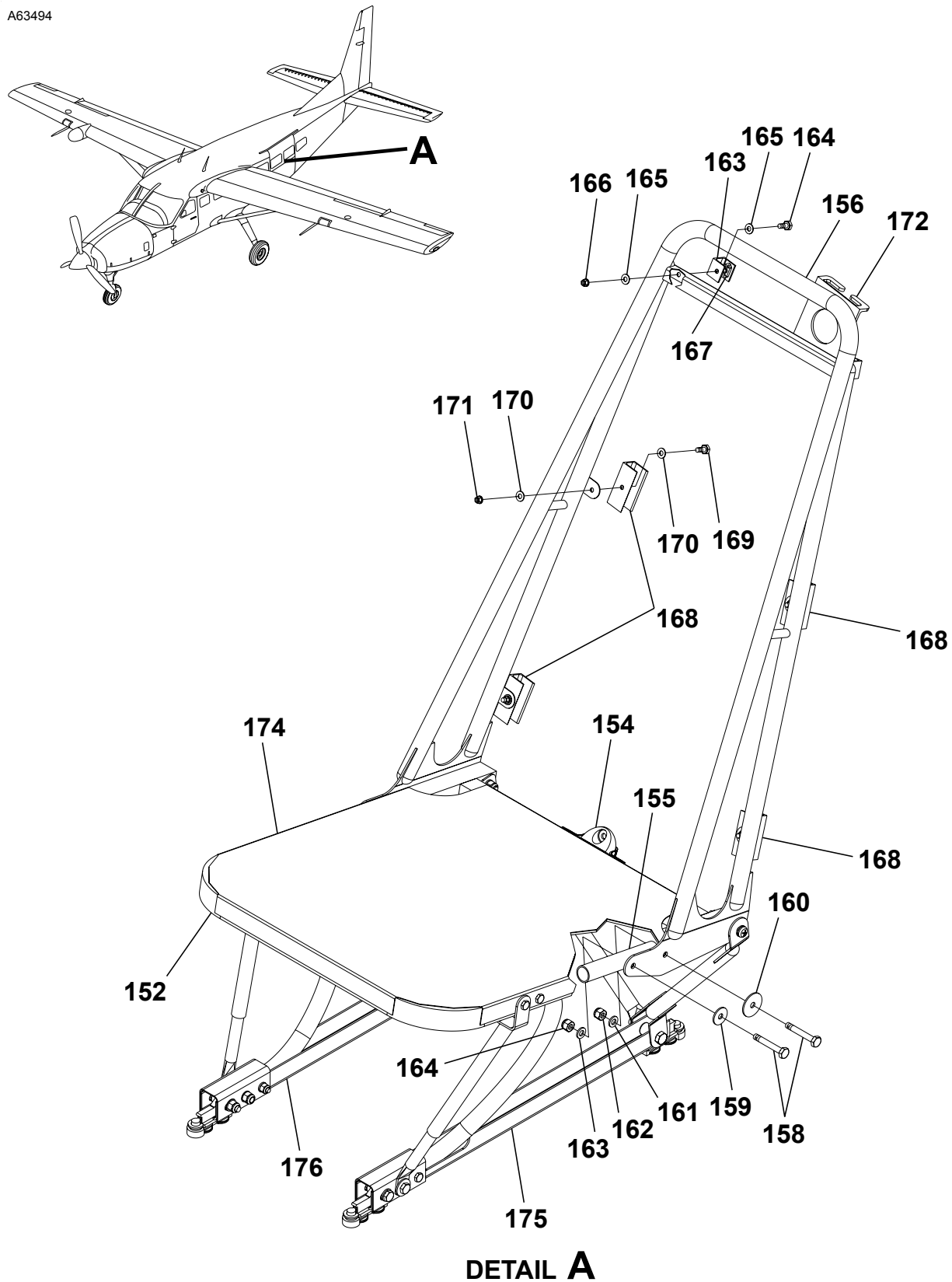
PASSENGER SEAT UPHOLSTERY AND STRUCTURE ASSEMBLY Figure 02A. (Sheet 3)
