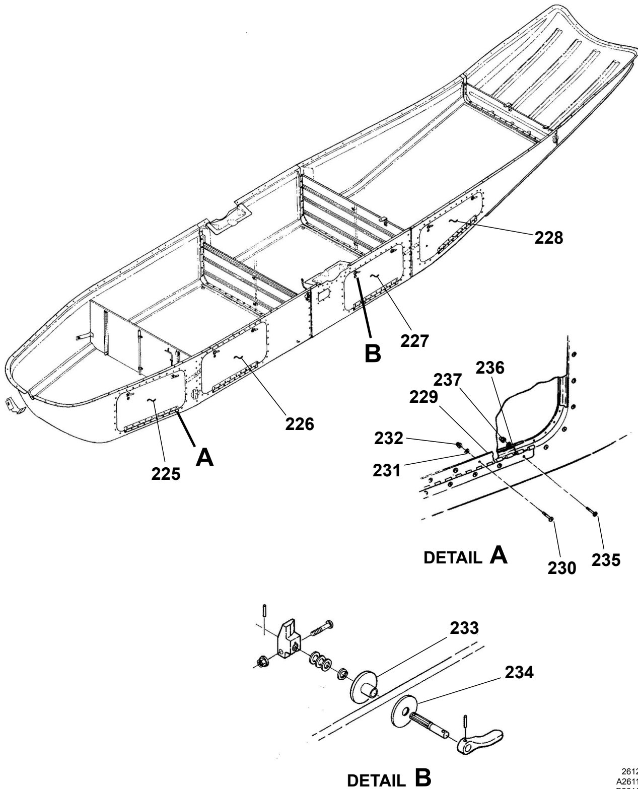
CARGO POD INSTALLATION Figure 02. (Sheet 4)
