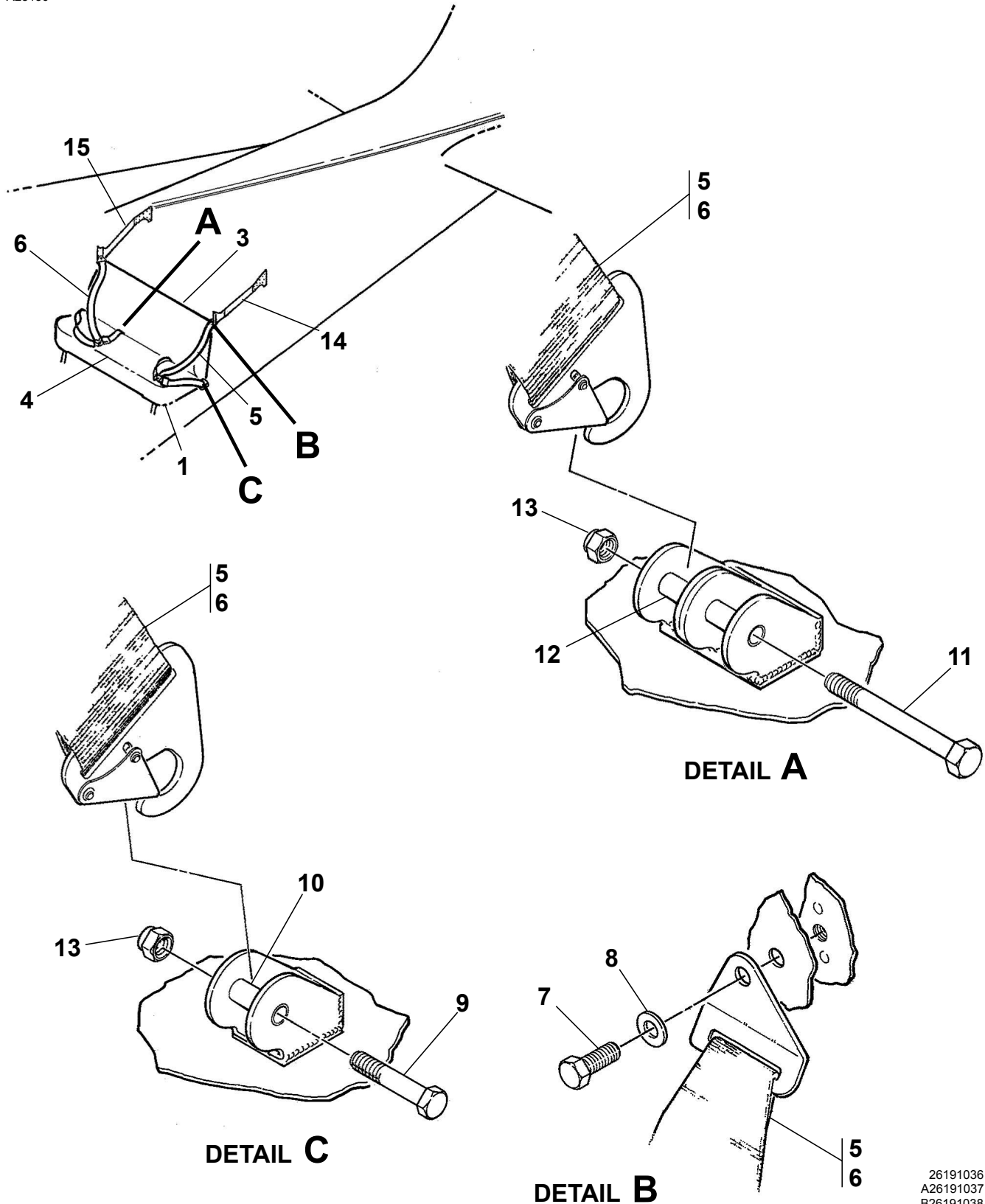
SEAT AND SHOULDER HARNESS INSTALLATION - 2 PASSENGER BRITISH CERTIFIED AIRPLANES Figure 02. (Sheet 1)
