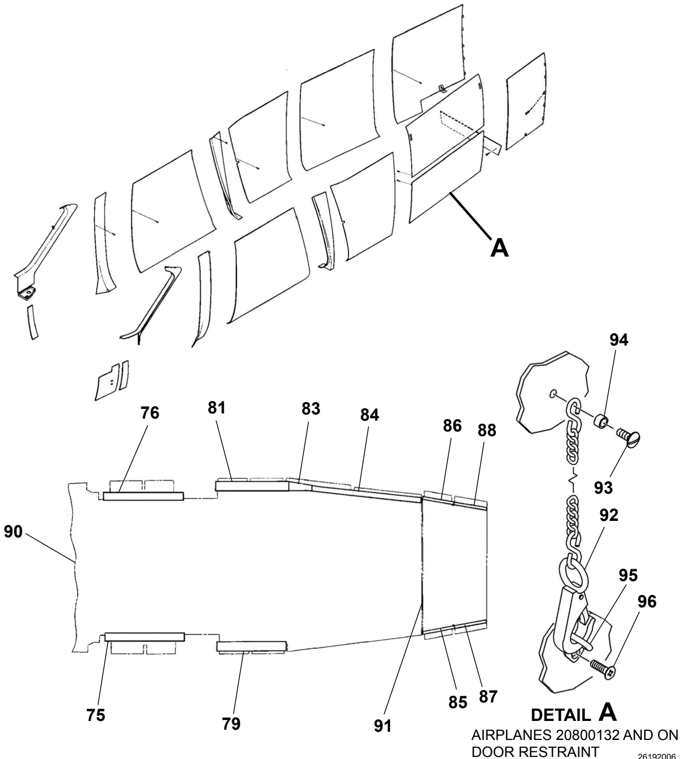
CABIN SIDEWALLS UPHOLSTERY Figure 03. (Sheet 2)
