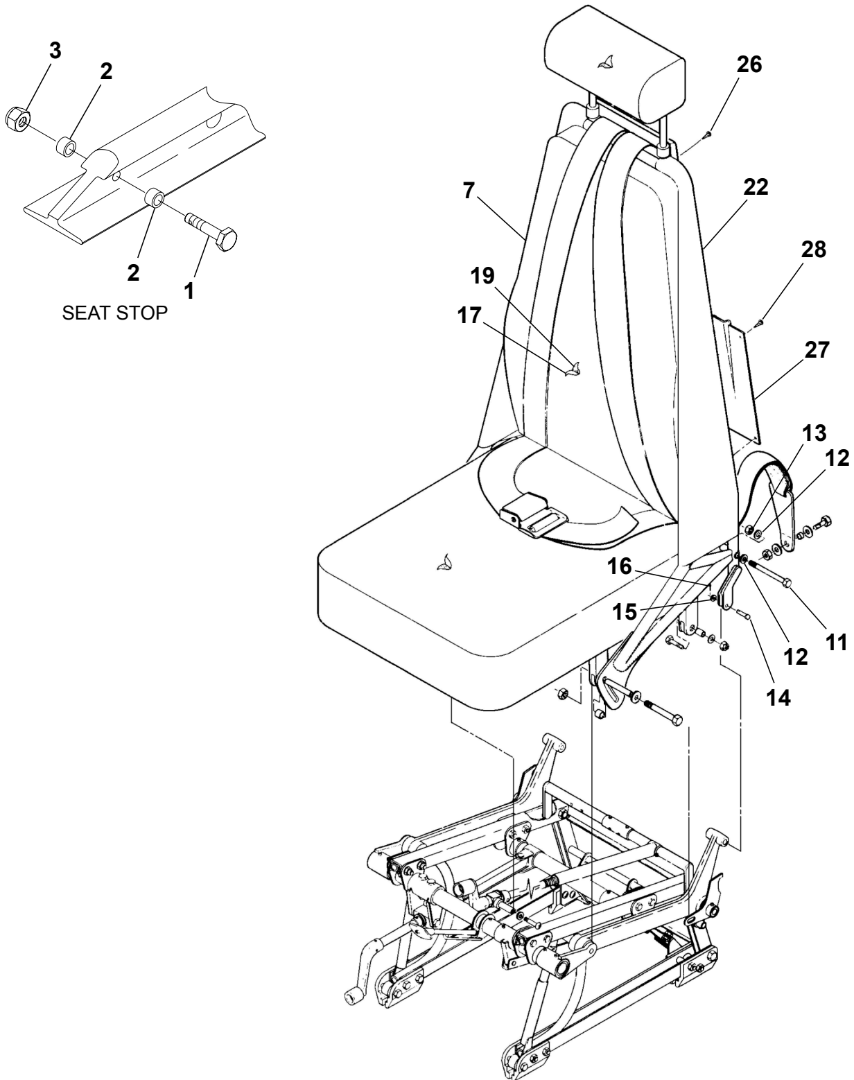
SEAT ASSEMBLY - PILOT AND COPILOT Figure 01. (Sheet 1)
