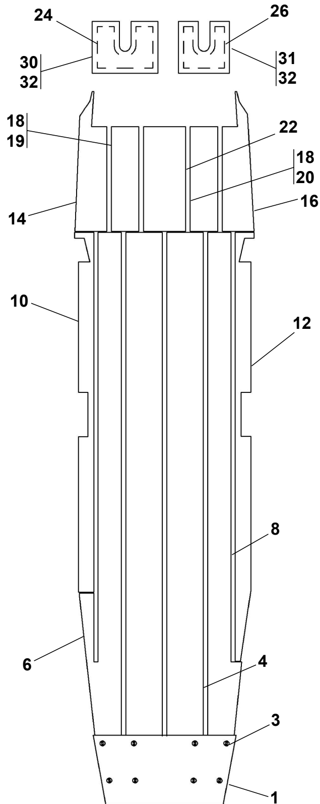
CABIN FLOOR COVERING AND CARPET INSTALLATION - PASSENGER VERSION Figure 04. (Sheet 1)
