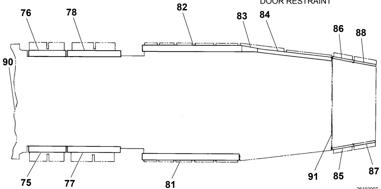
CABIN SIDEWALLS UPHOLSTERY Figure 04. (Sheet 2)
