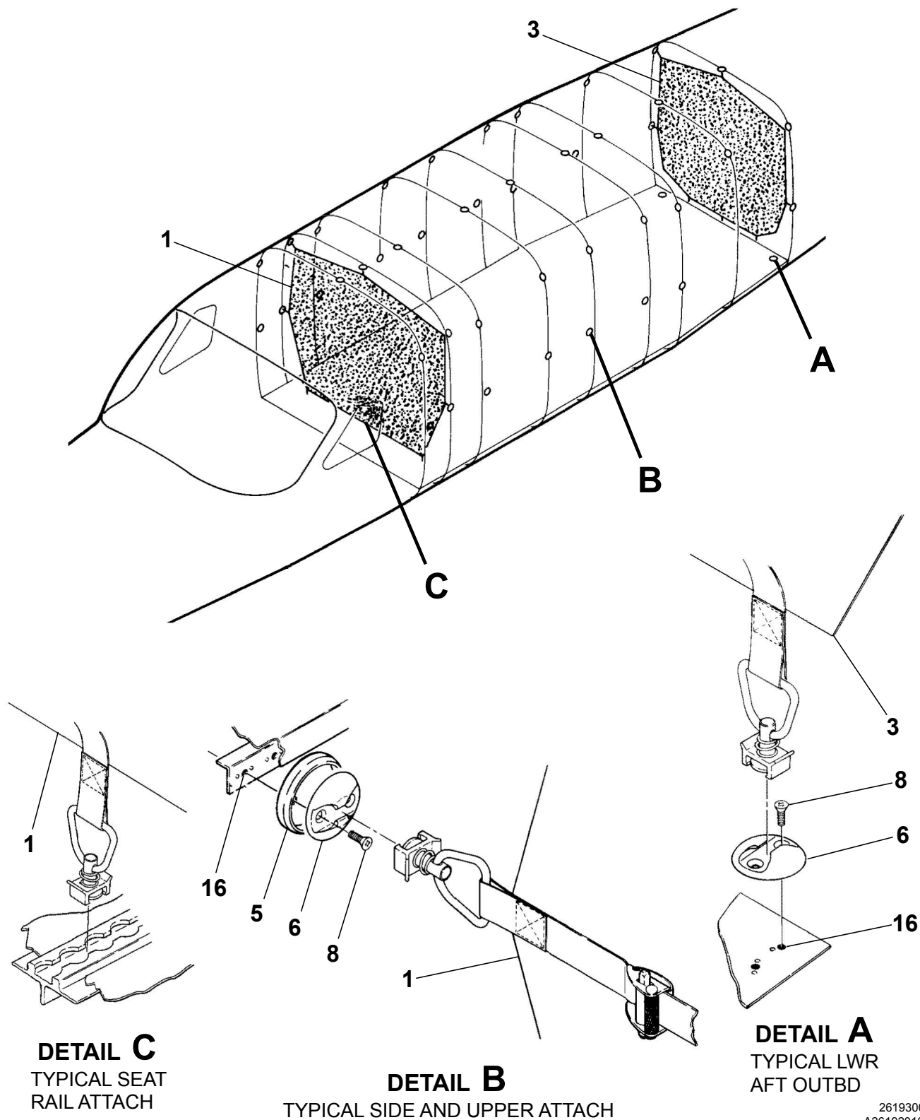
CARGO PARTITION INSTALLATION WITH CARGO TIEDOWN Figure 03. (Sheet 1)
