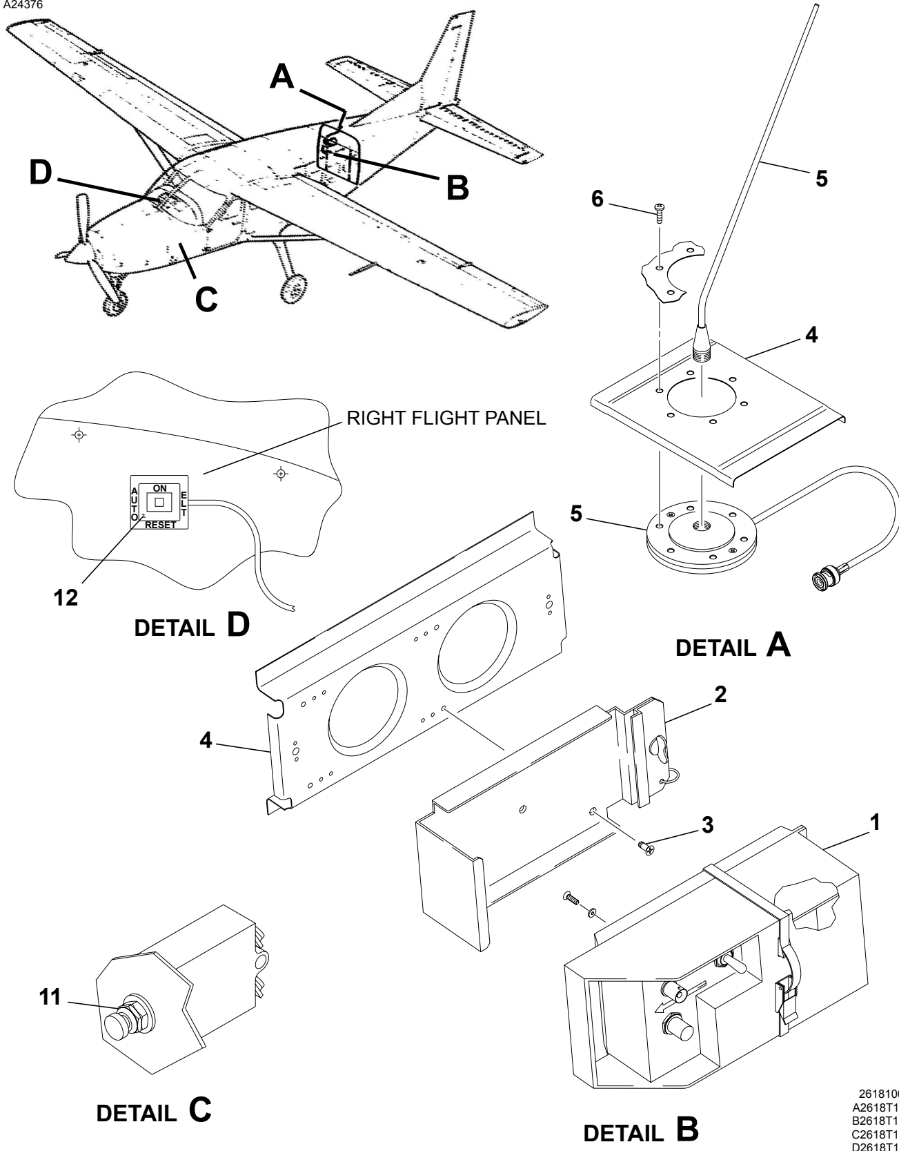
EMERGENCY LOCATOR TRANSMITTER INSTALLATION - POINTER 3000-11 Figure 03. (Sheet 1)
