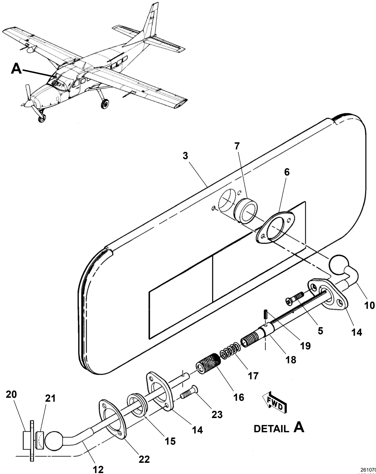
SUNVISOR INSTALLATION Figure 01. (Sheet 1)
