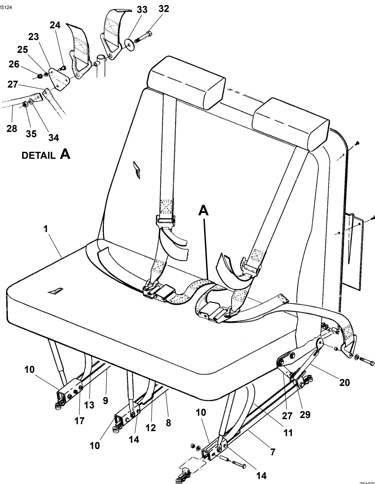
SEAT ASSEMBLY - BENCH Figure 03. (Sheet 1)
