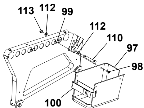
DETAIL D
