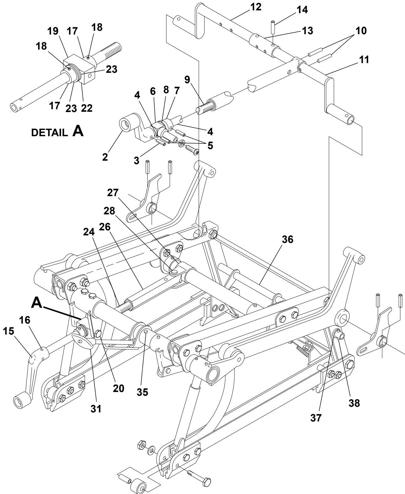
PEDESTAL ASSEMBLY - PILOT AND COPILOT SEAT Figure 03. (Sheet 1)
