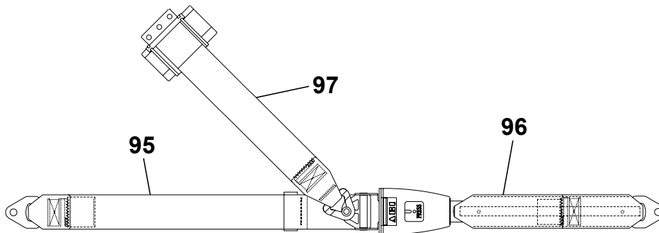
DETAIL C
