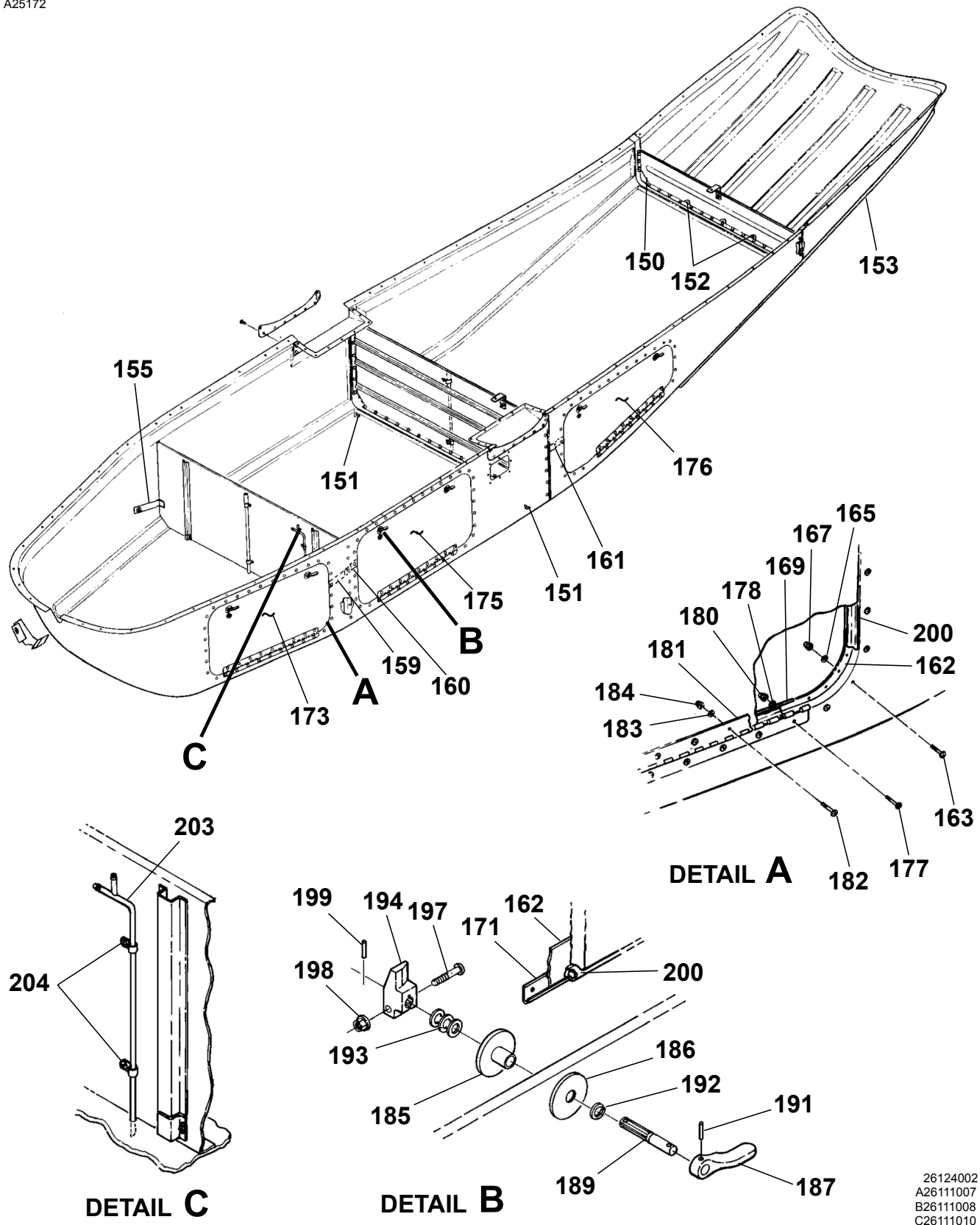
CARGO POD INSTALLATION Figure 01. (Sheet 3)
