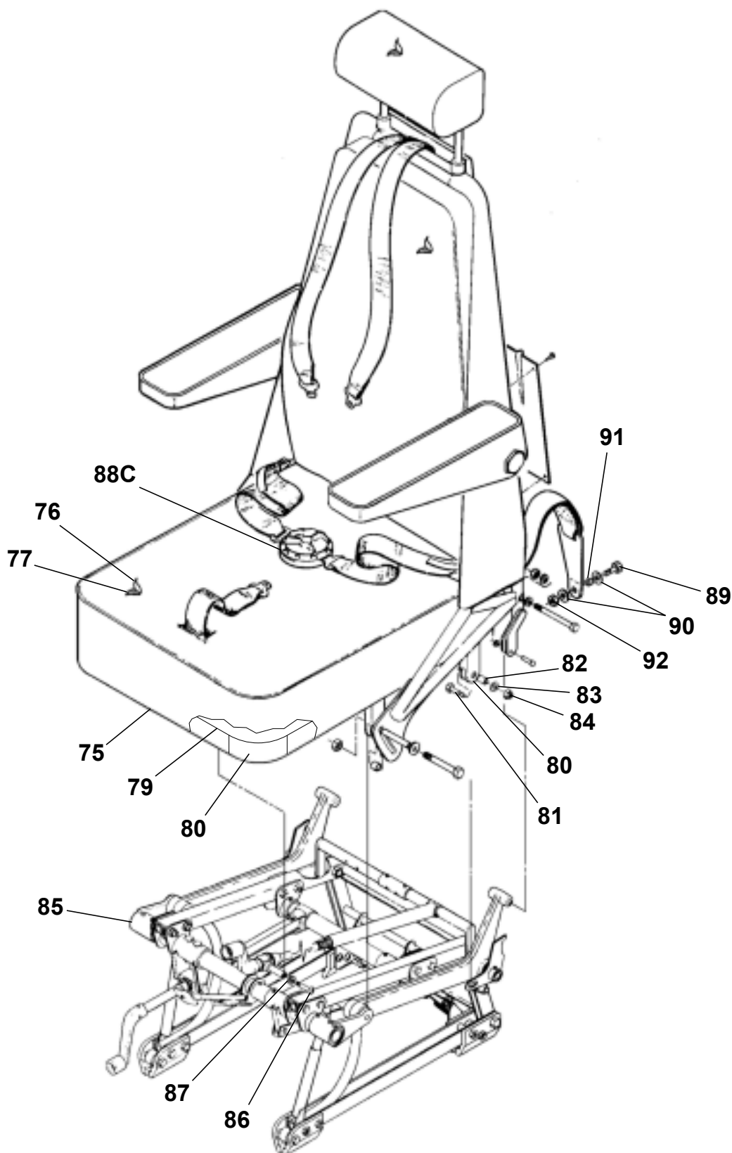
SEAT ASSEMBLY - PILOT AND COPILOT WITH ARMREST Figure 02. (Sheet 2)
