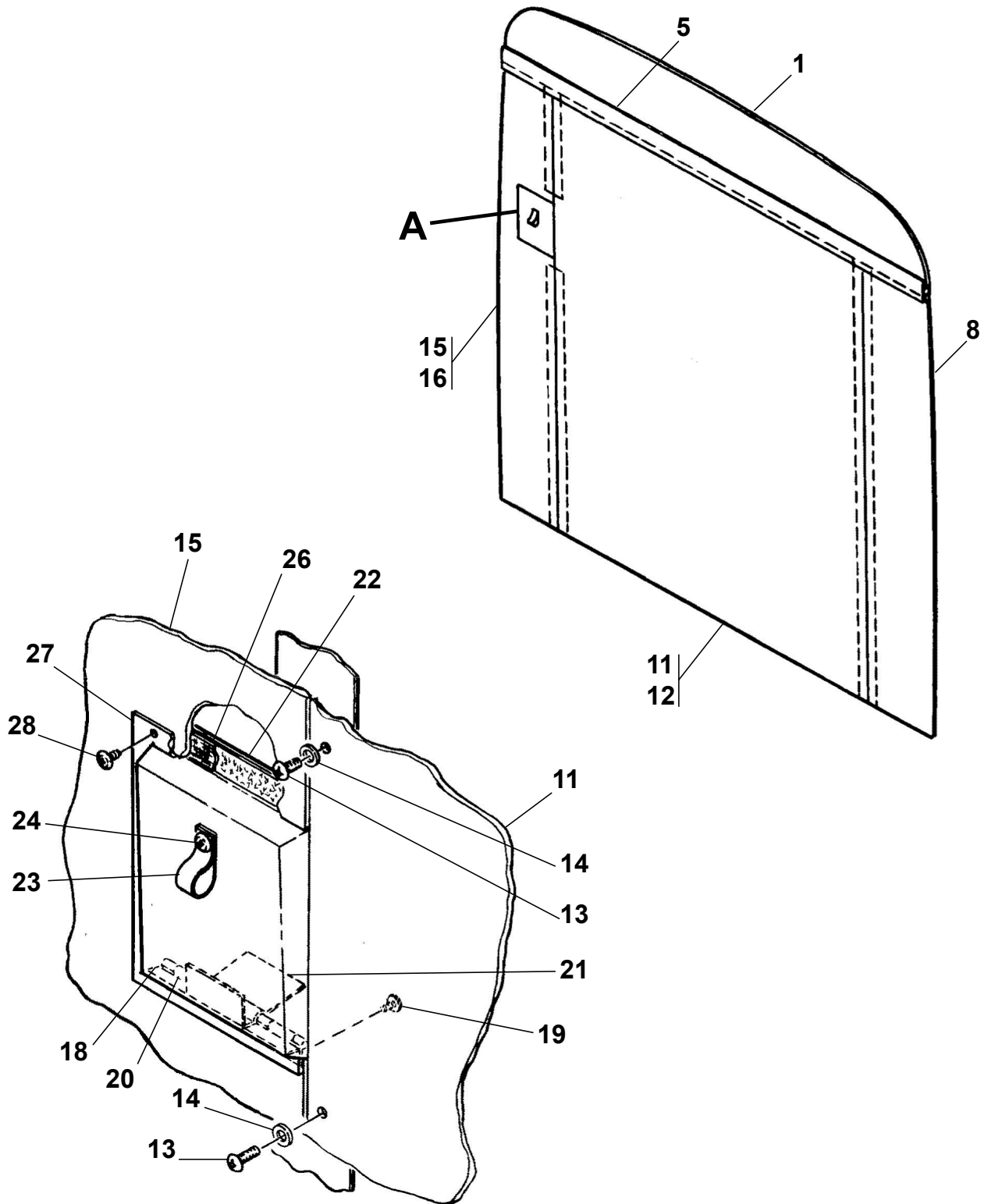
REAR CARGO COMPARTMENT WALL UPHOLSTERY - HARD INTERIOR Figure 02. (Sheet 1)
