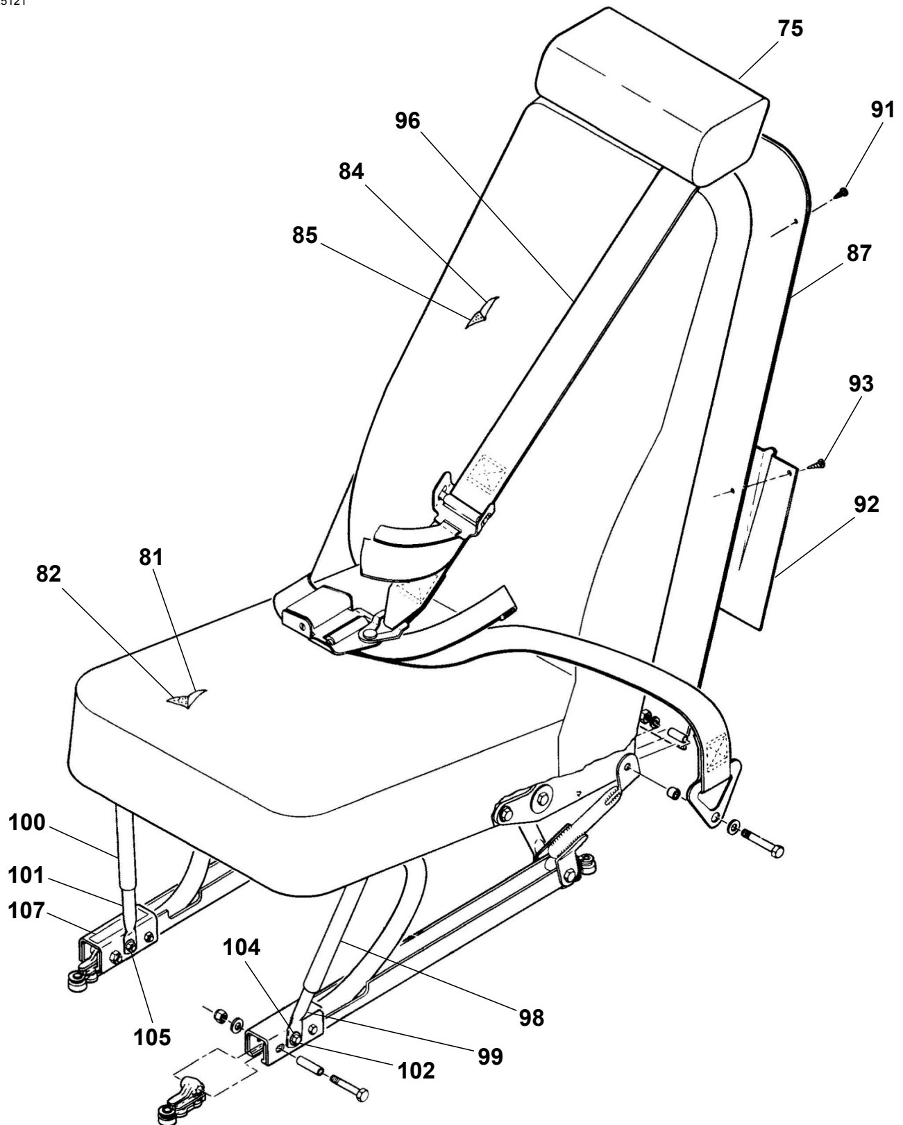
SEAT ASSEMBLY - SINGLE LH Figure 01. (Sheet 2)
