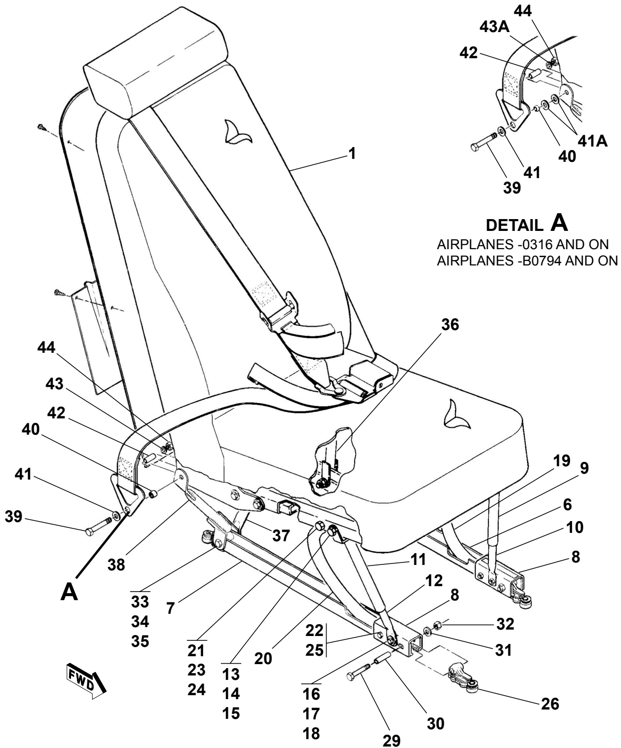
SEAT ASSEMBLY - SINGLE RH Figure 02. (Sheet 1)
