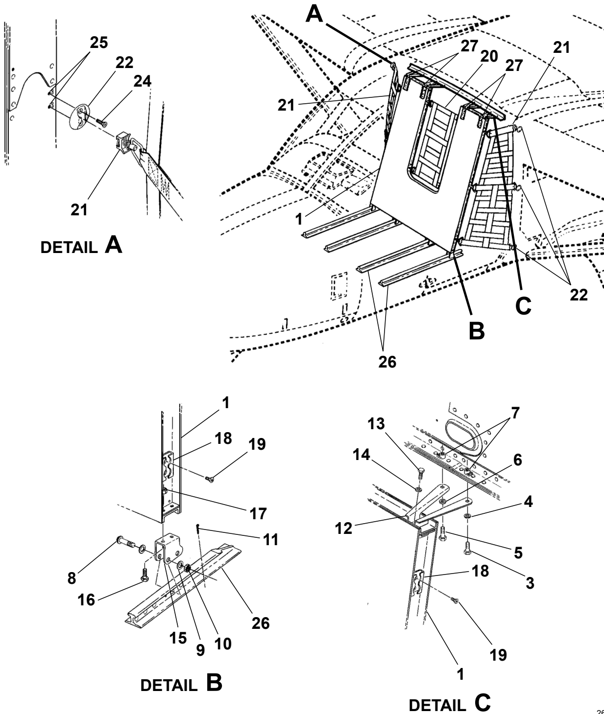
CARGO BARRIER INSTALLATION Figure 01. (Sheet 1)
