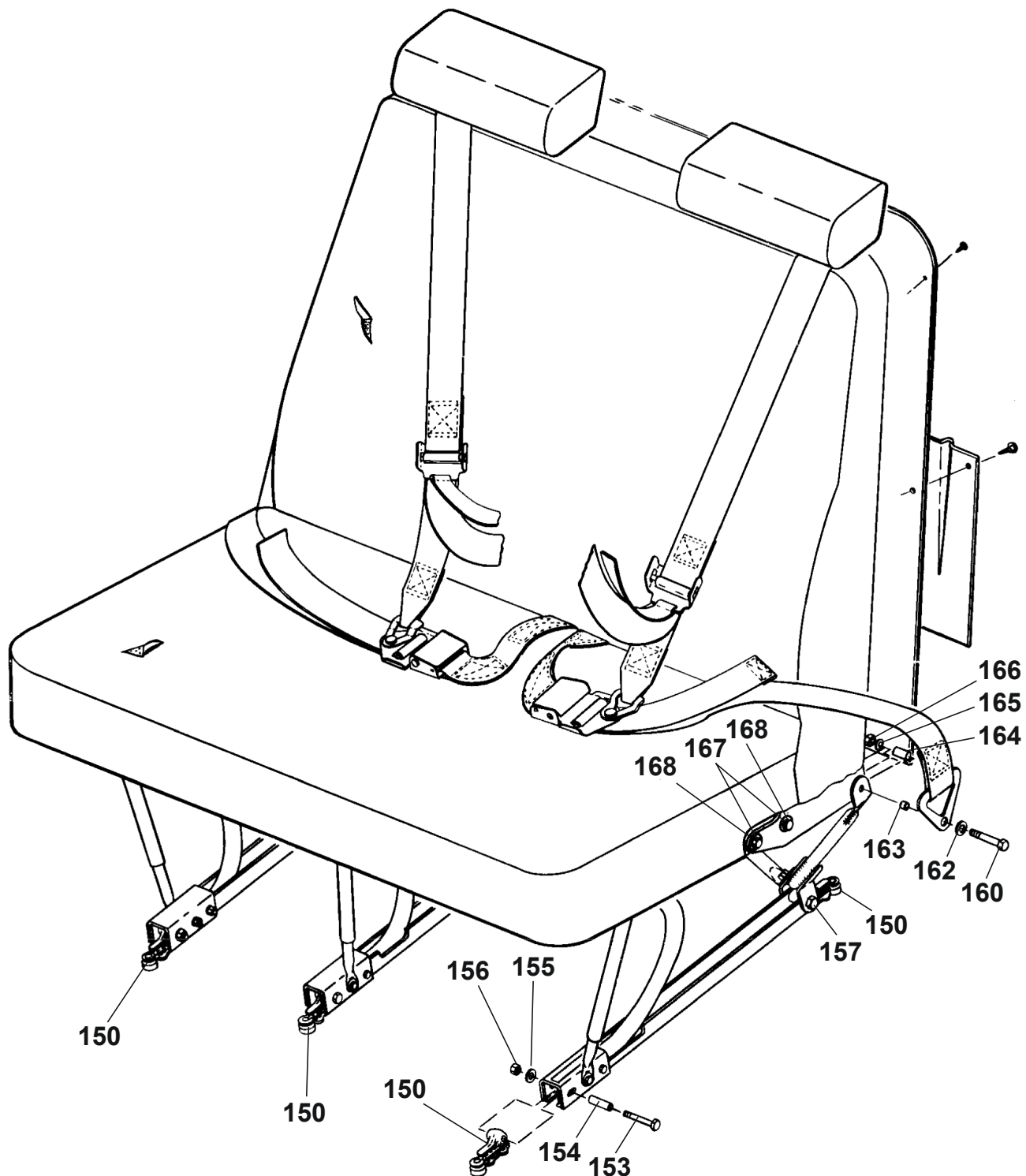
SEAT ASSEMBLY - BENCH Figure 03. (Sheet 3)
