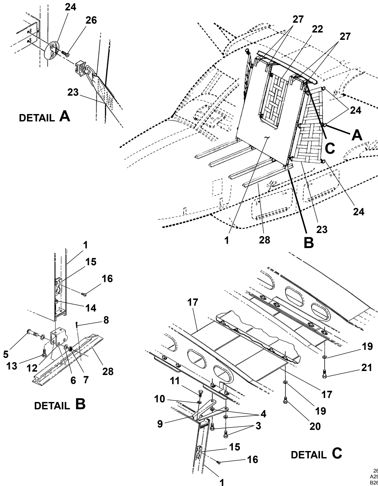
CARGO BARRIER INSTALLATION Figure 02. (Sheet 1)
