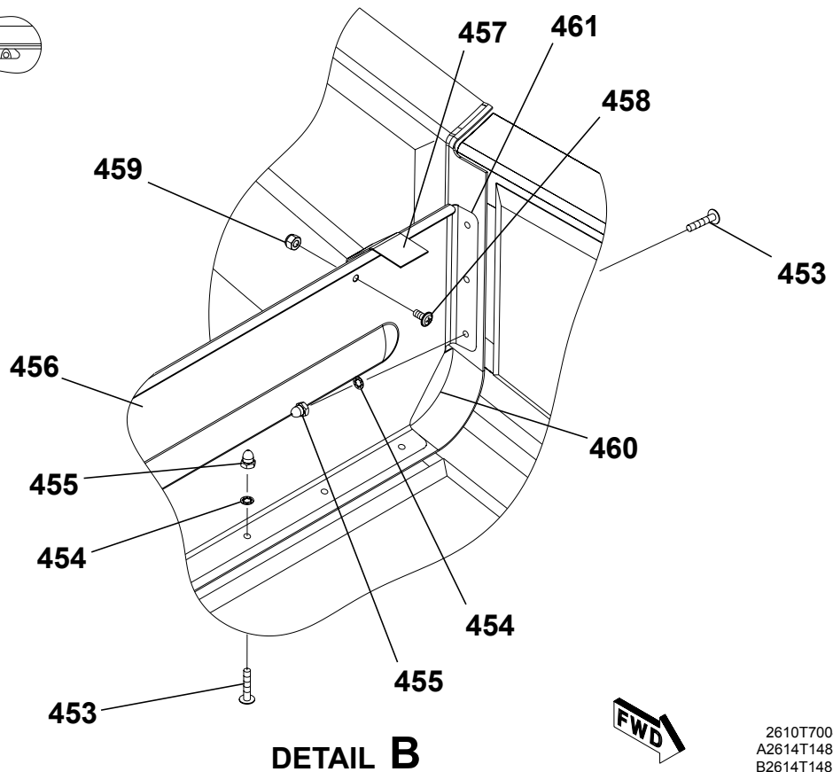
CARGO POD FIELD INSTALLATION Figure 02A. (Sheet 7)
