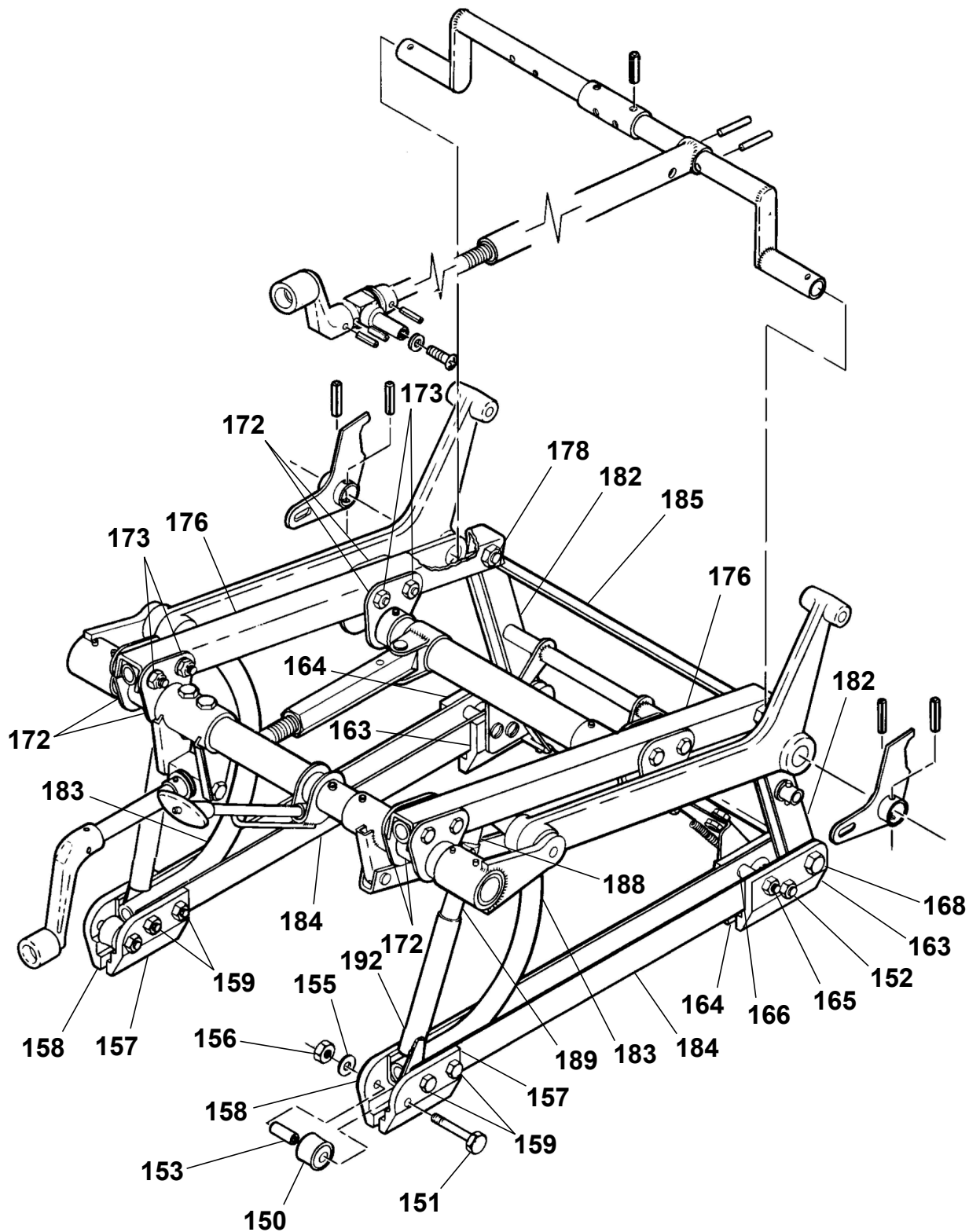
PEDESTAL ASSEMBLY - PILOT AND COPILOT SEAT Figure 03. (Sheet 3)
