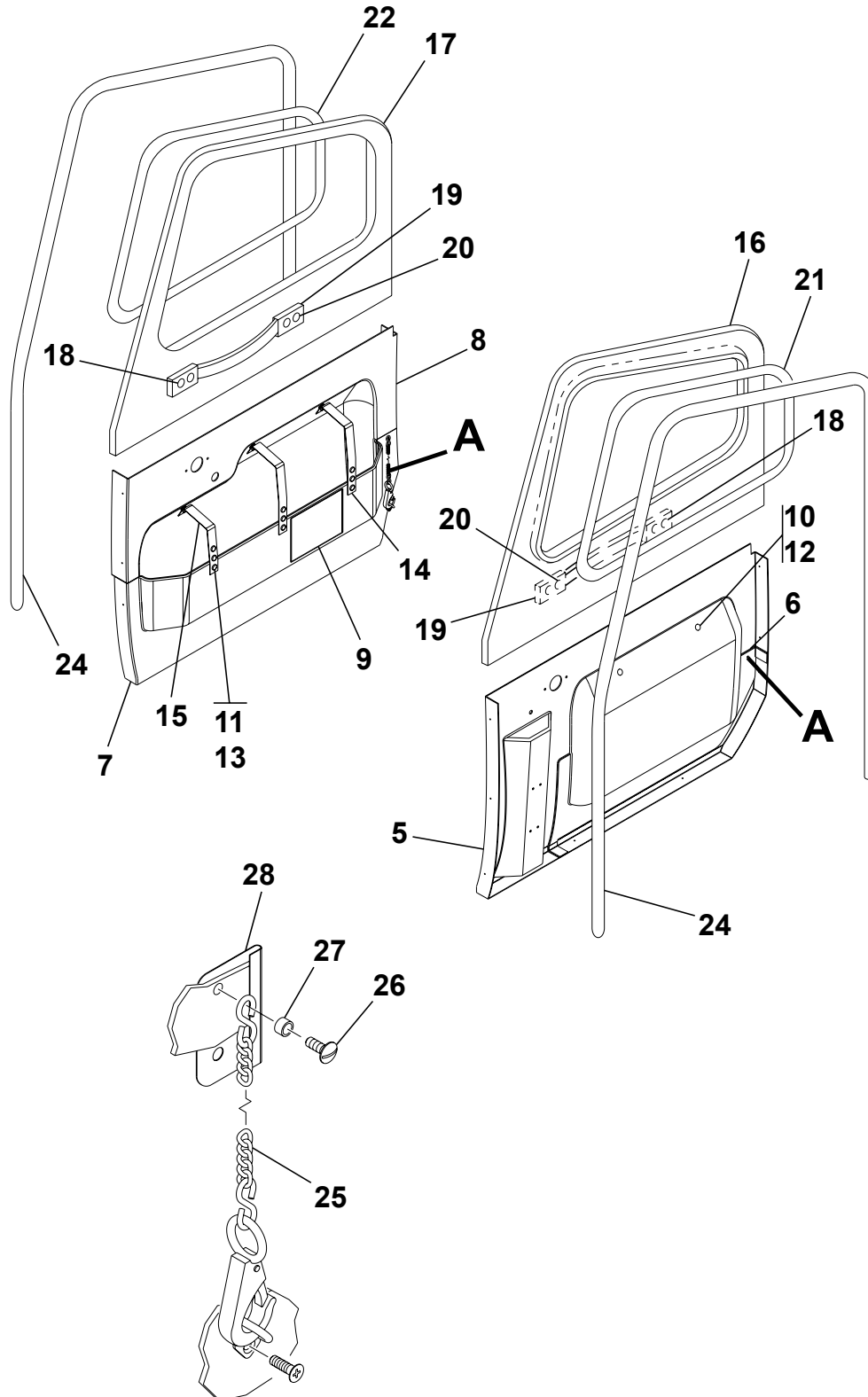
PILOT AND COPILOT DOOR UPHOLSTERY Figure 01A. (Sheet 1)
