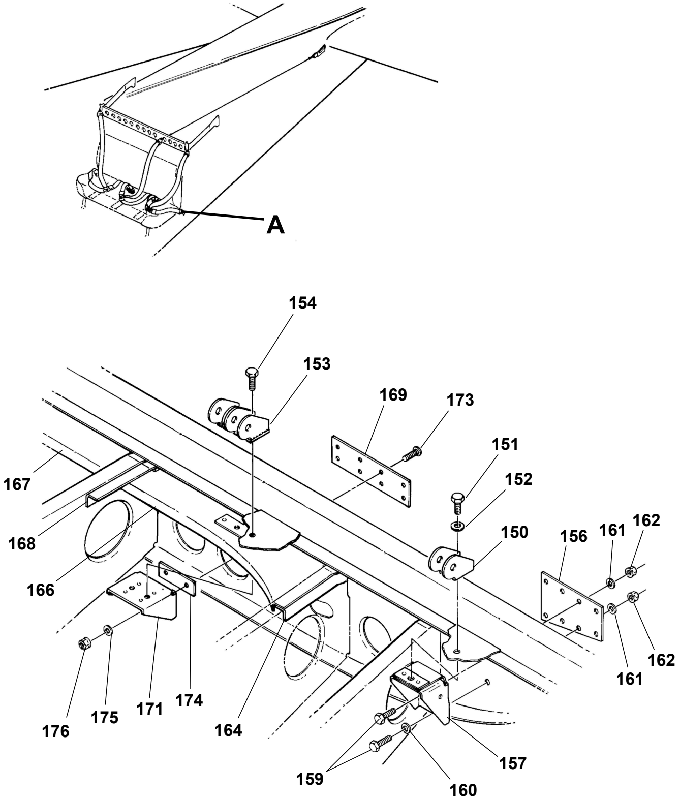
SEAT AND SHOULDER HARNESS INSTALLATION - 3 PASSENGER Figure 01. (Sheet 3)
