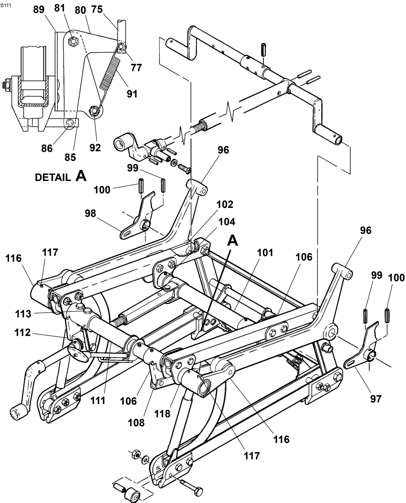
PEDESTAL ASSEMBLY - PILOT AND COPILOT SEAT Figure 03. (Sheet 2)
