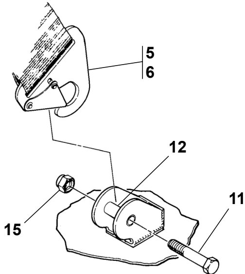
DETAIL D
