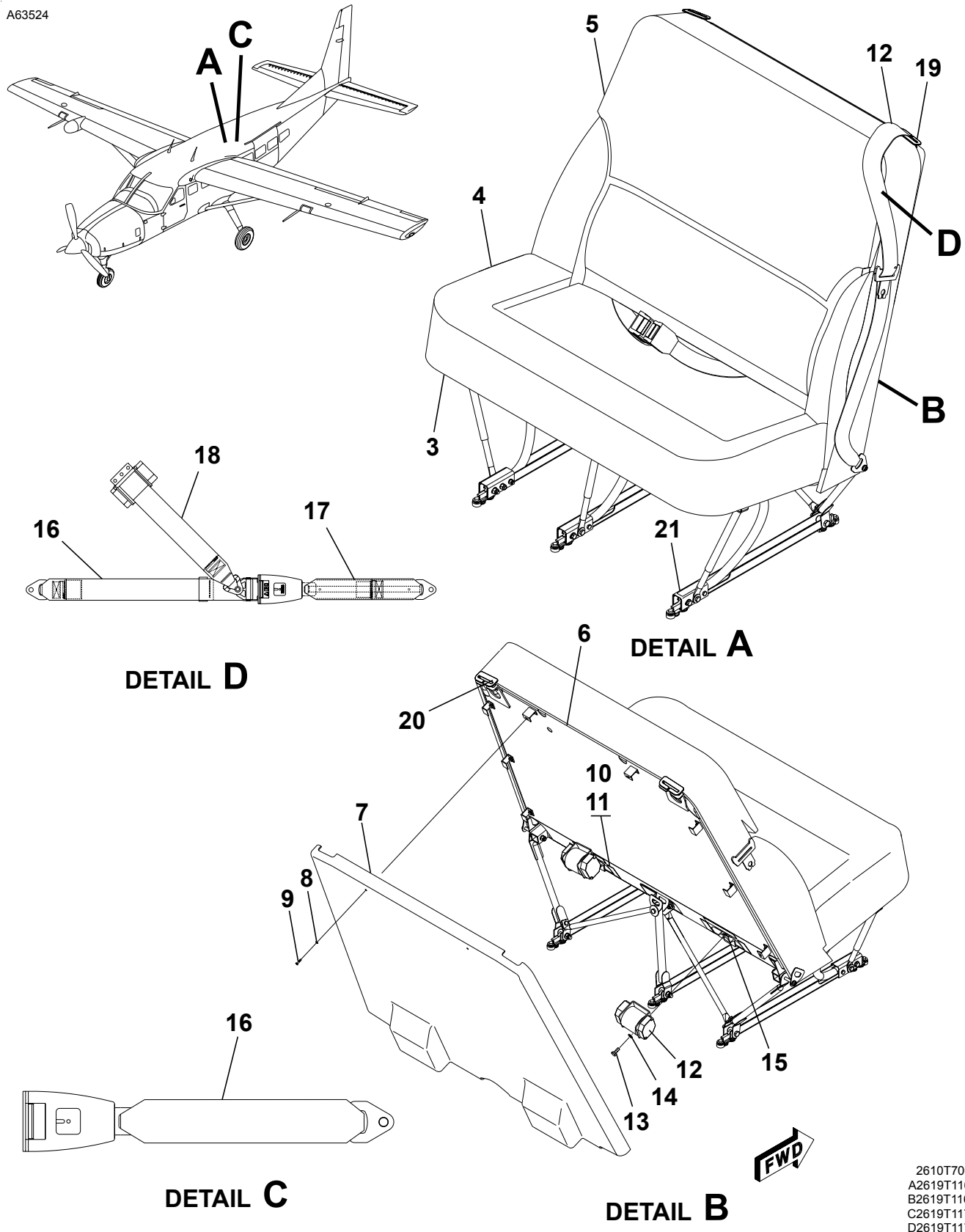
BENCH SEAT UPHOLSTERY AND STRUCTURE ASSY Figure 01. (Sheet 1)
