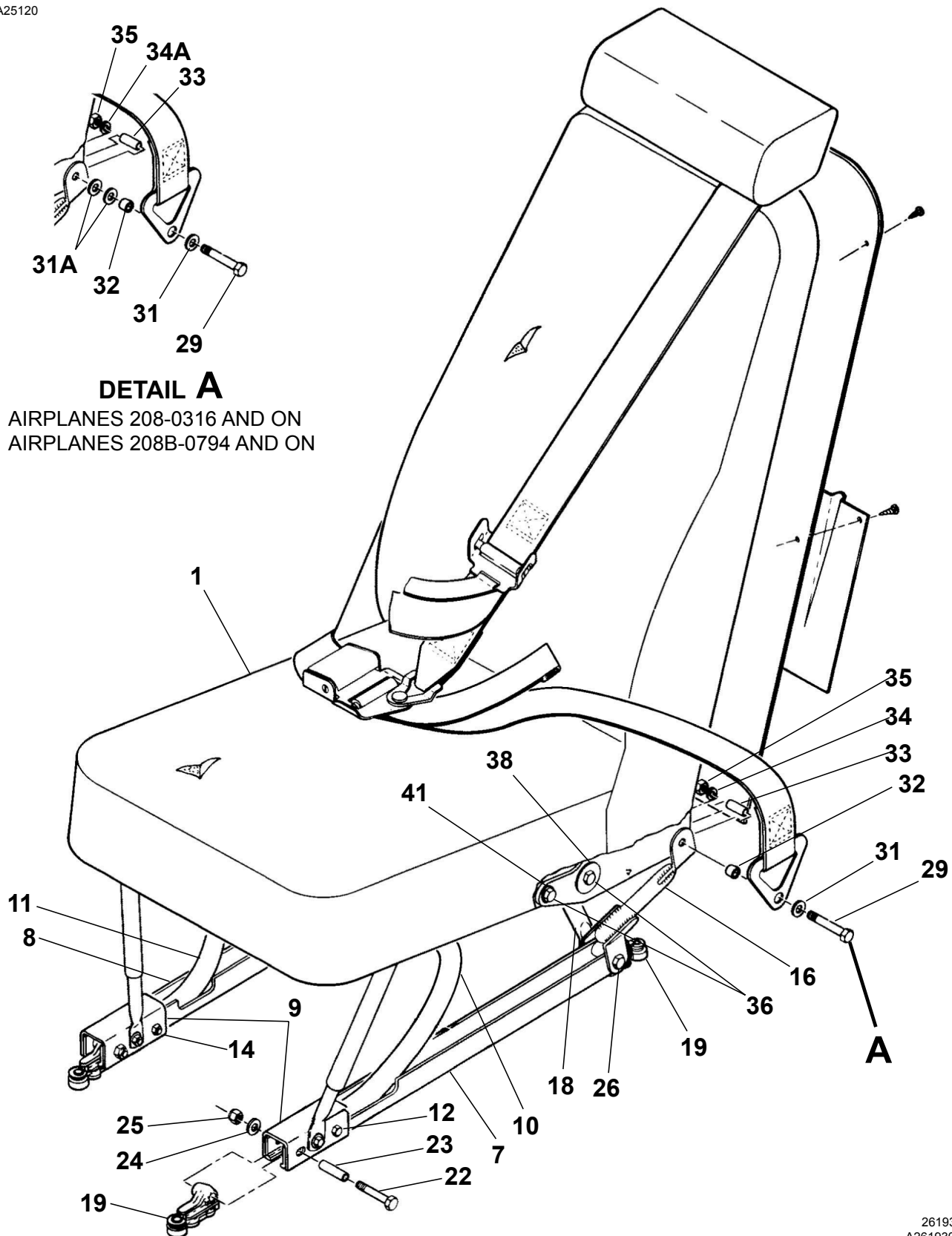
SEAT ASSEMBLY - SINGLE LH Figure 01. (Sheet 1)
