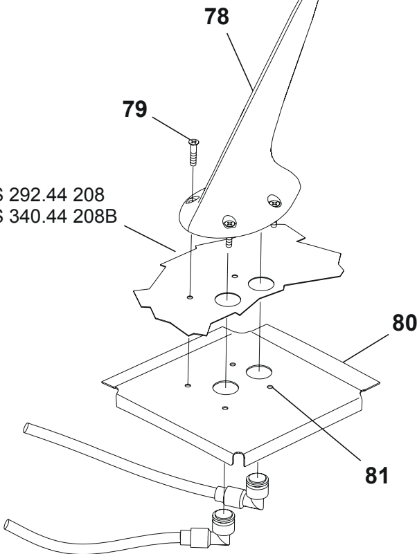
DETAIL C
