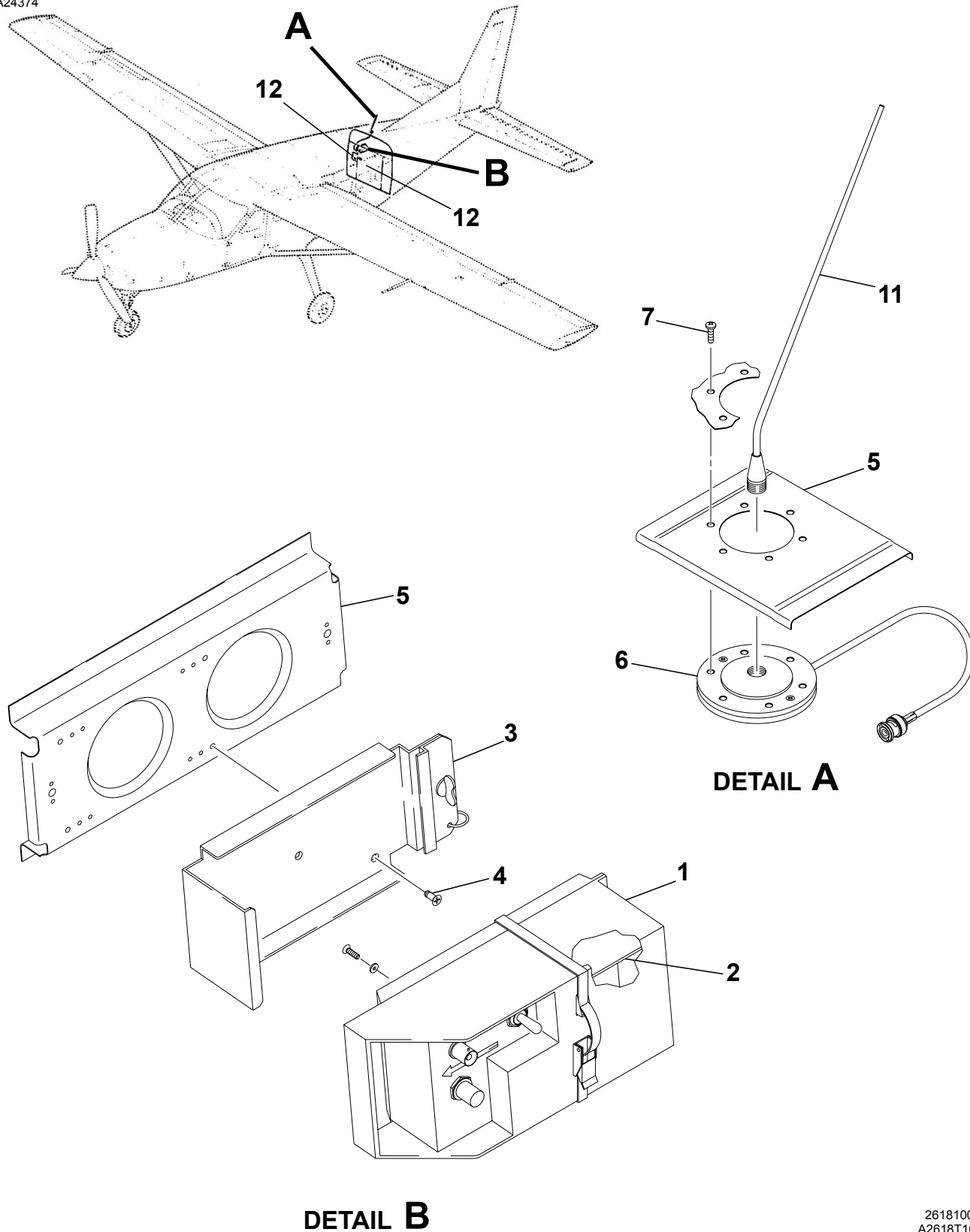
EMERGENCY LOCATOR TRANSMITTER INSTALLATION - POINTER 3000 Figure 02. (Sheet 1)
