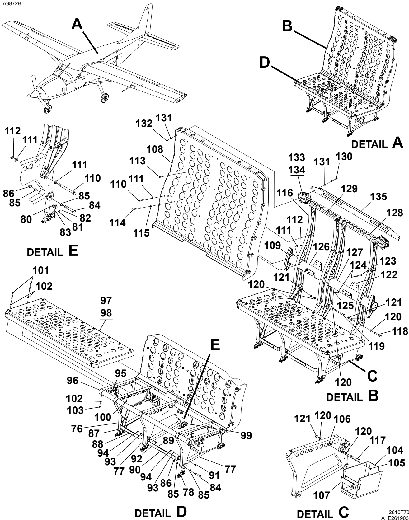
BENCH SEAT UPHOLSTERY AND STRUCTURE ASSY Figure 02. (Sheet 2)
