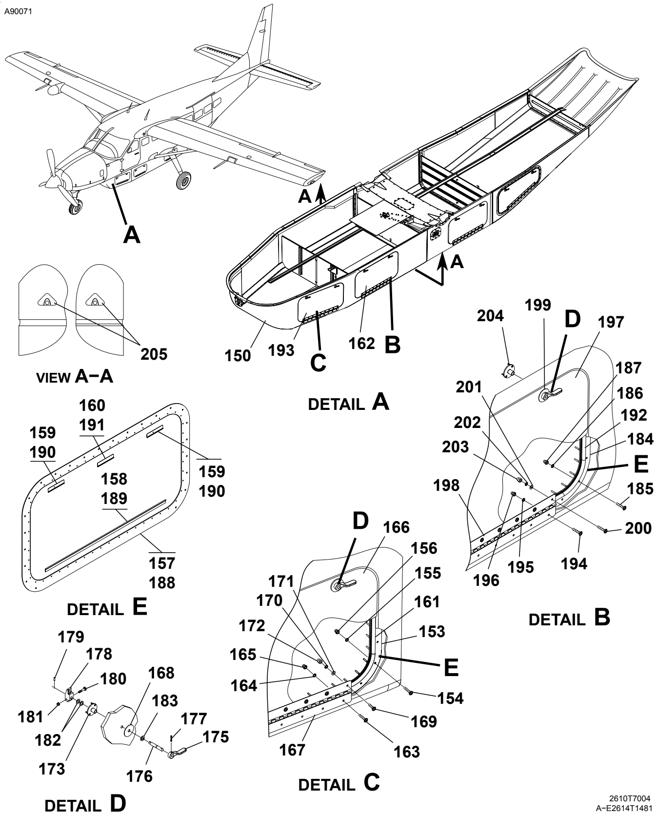
CARGO POD FIELD INSTALLATION Figure 02A. (Sheet 3)
