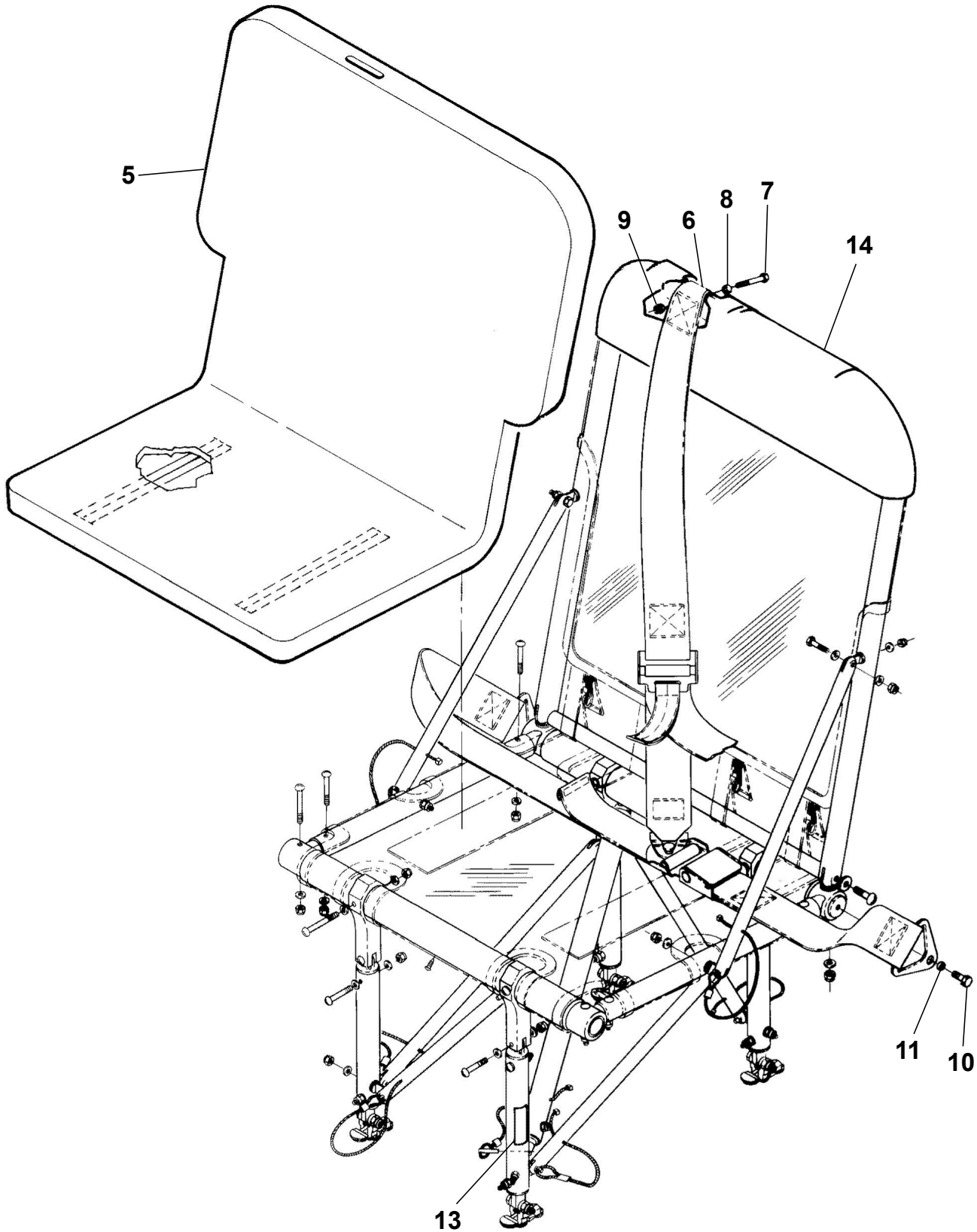
FOLDING UTILITY STYLE SEAT INSTALLATION Figure 01. (Sheet 1)
